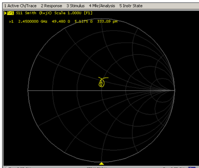
Impedance Test-Body
