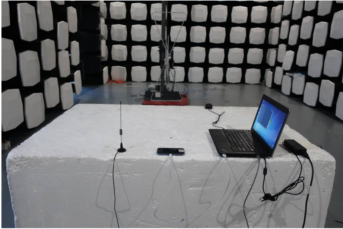
Radiated Disturbance (30MHz-1GHz)
