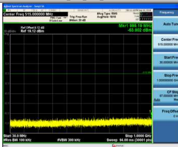
11G_Ant2_2417_30~1000
