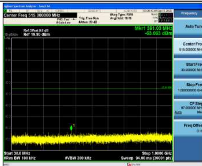
11N40SISO_Ant1_2432_30~1000
