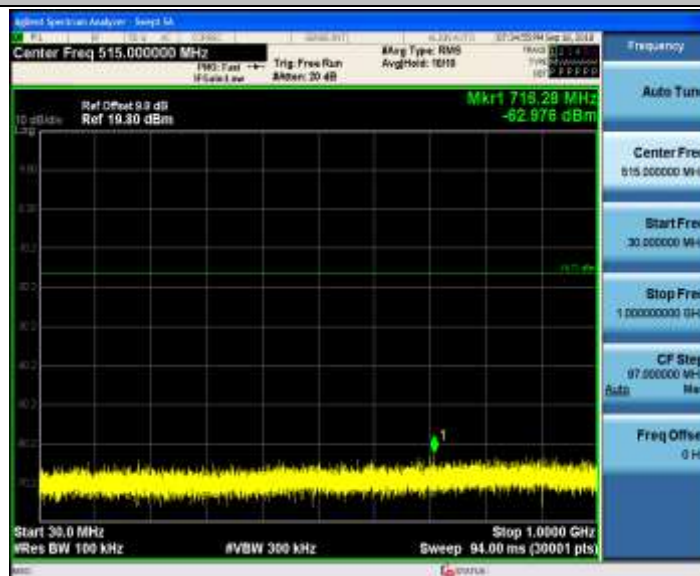
11G_Ant1_2457_30~1000
