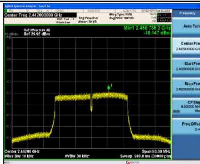
11N40SISO_Ant1_2442
