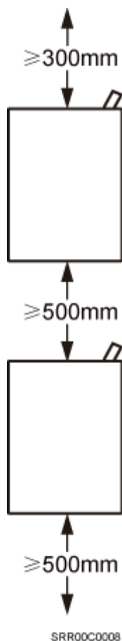
Figure 3-33 Recommended vertical spacing between RRUs
