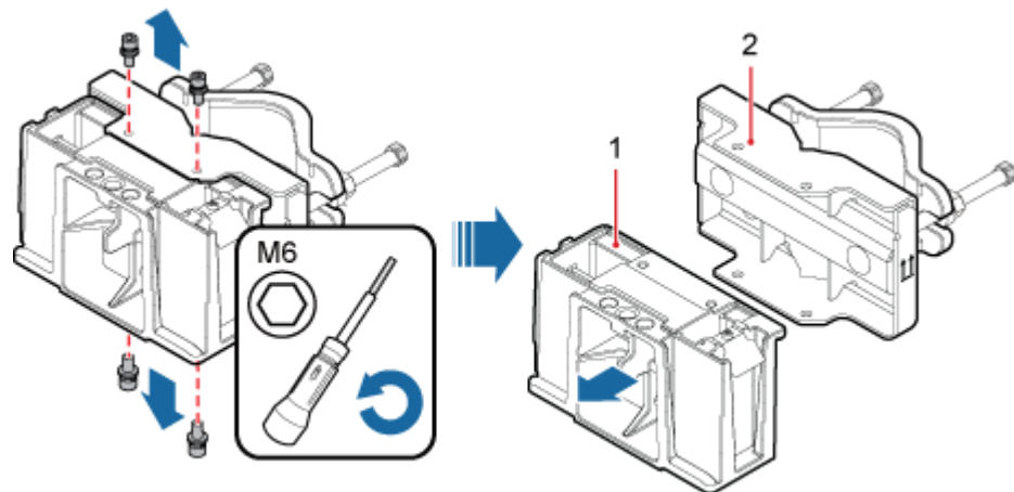
Figure 8-9 Removing the RRU main bracket
