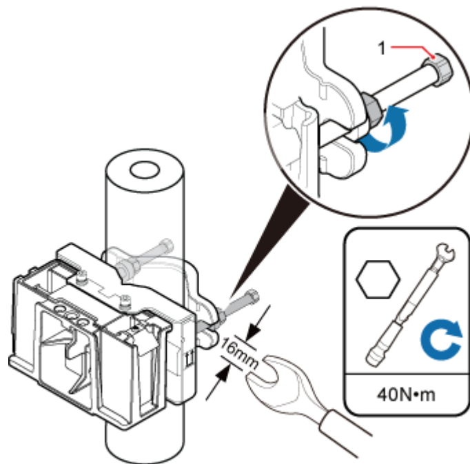
Figure 8-5 Securing the RRU mounting brackets
