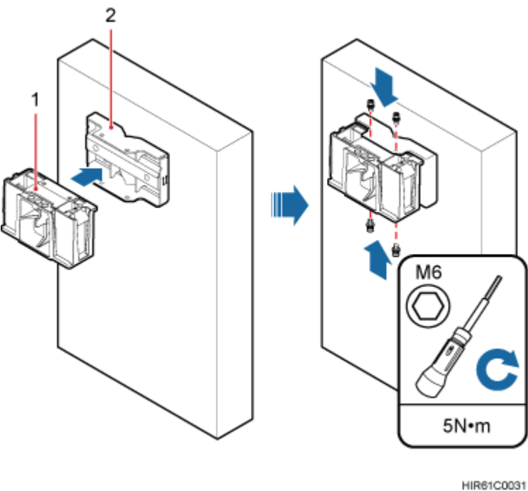
Figure 8-40 Installing the main bracket
