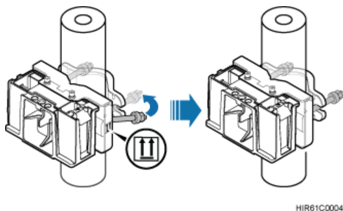
Figure 8-4 Installing the RRU mounting brackets
