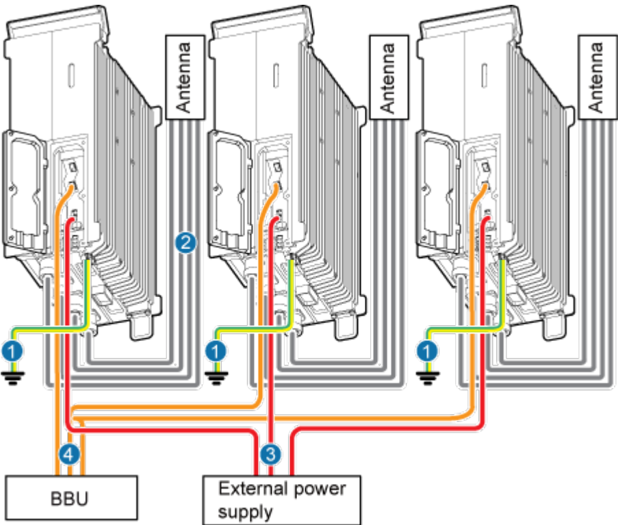
Figure 9-10 Cable connections of multiple single-mode RRUs
