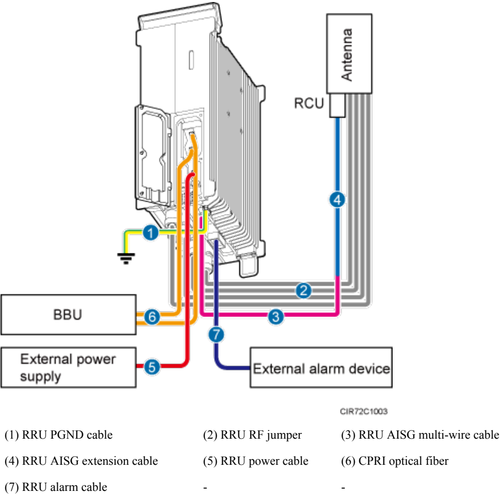
Figure 9-9 Cable connections of a multimode RRU
