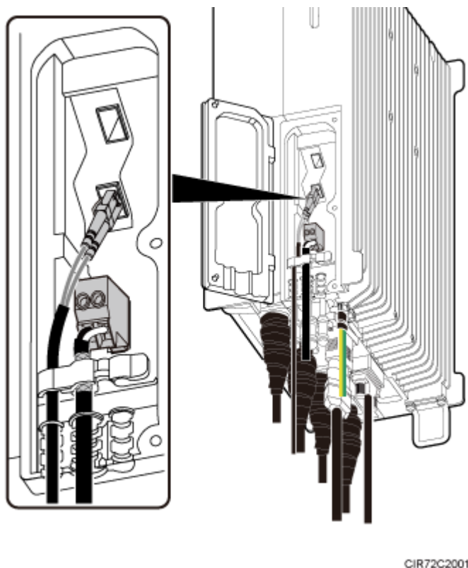
Figure 9-29 Installing an RRU power cable
