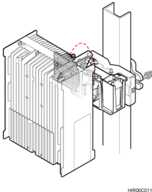
Figure 8-27 Installing the RRU onto the main bracket
