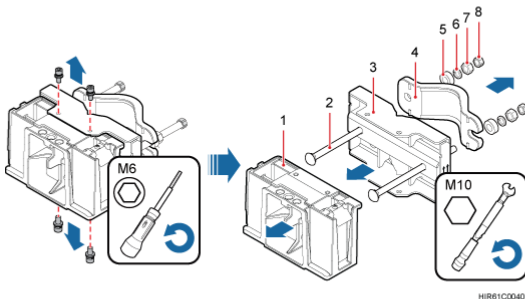
Figure 8-36 Disassembling the RRU mounting brackets
