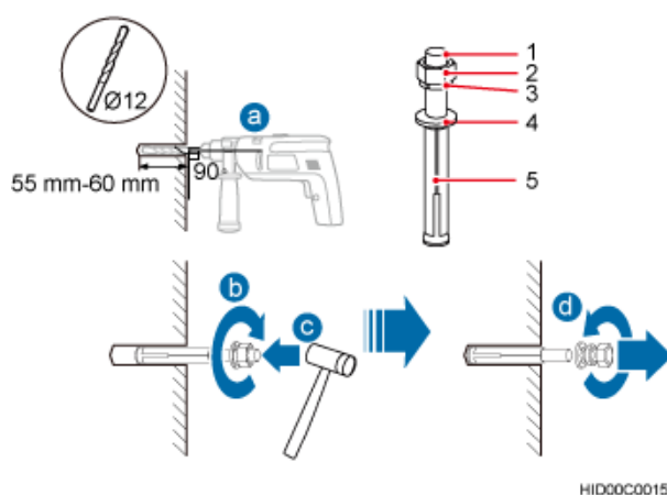
Figure 8-38 Drilling holes and inserting expansion anchor bolts
