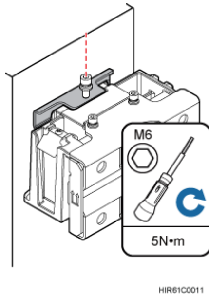
Figure 8-7 Securing the captive screw into the connection hole
