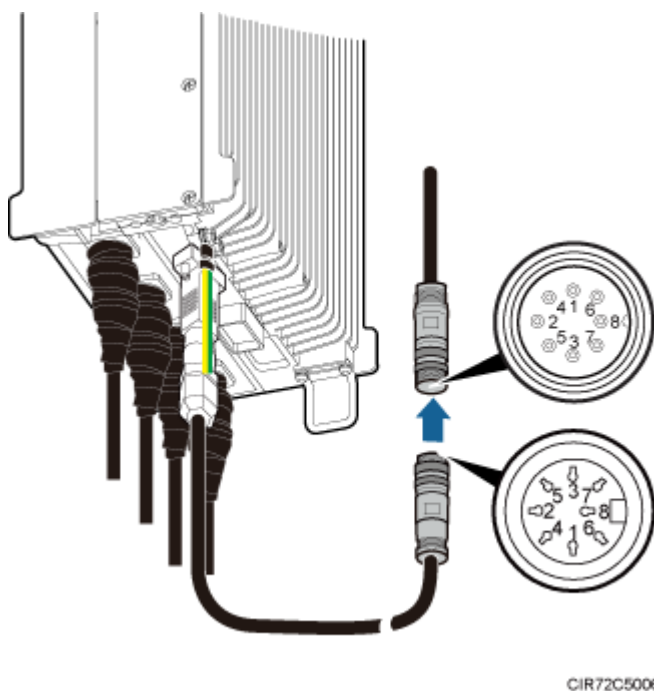
Figure 9-21 Installing an RRU AISG multi-wire cable
