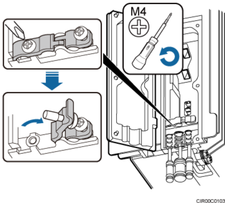
Figure 9-26 Opening clips
