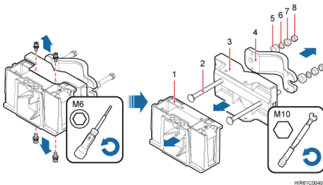
Figure 8-44 Disassembling the RRU mounting brackets
