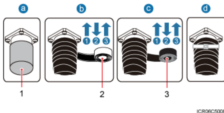
Figure 9-18 Waterproofing a dustproof cap
