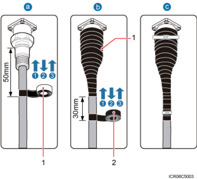
Figure 9-17 Waterproofing a connector of the RF jumper
