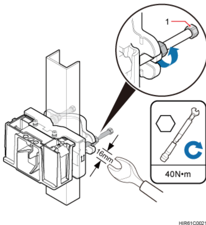
Figure 8-25 Securing the RRU mounting brackets
