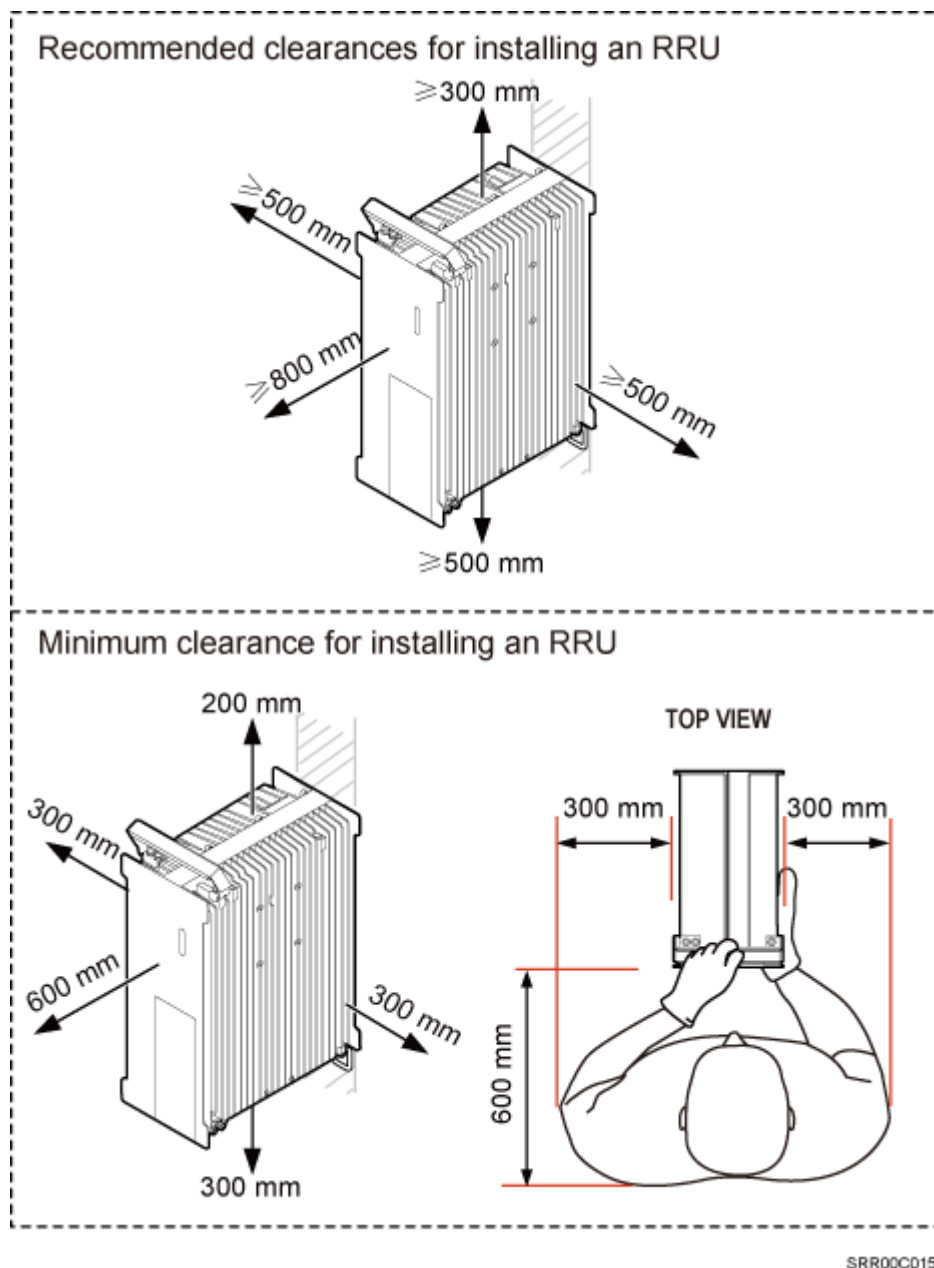
Figure 3-22 Clearance for a single RRU in side-mounted mode
