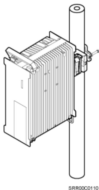
Figure 3-8 A single RRU installed on a pole
