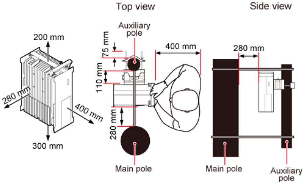
Figure 3-25 Minimum clearance for a single RRU in standard or reverse mode on a tower
