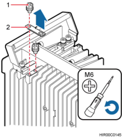
Figure 6-1 Removing the metal sheet
