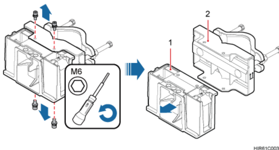
Figure 8-16 Removing the RRU main bracket
