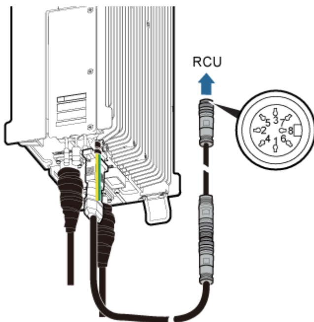
Figure 9-19 Installing an inter-RRU RF cable
