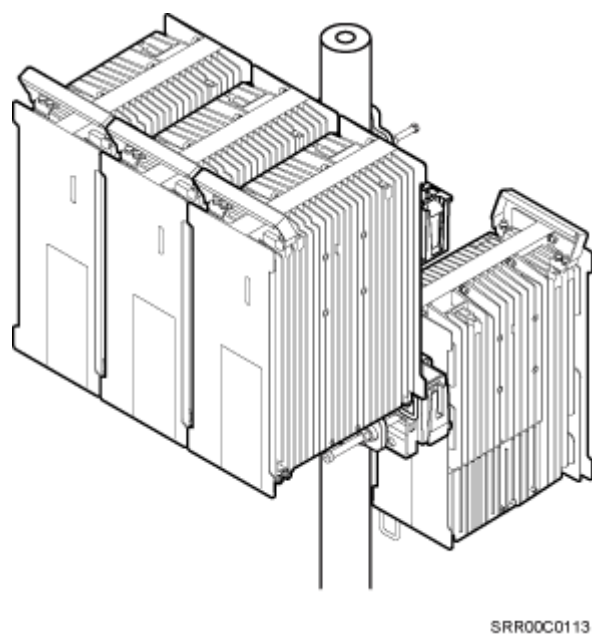
Figure 3-11 Four RRUs installed on a pole
