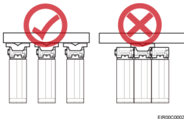
Figure 3-19 Correct installation of mounting brackets for RRUs installed on an IFS06
