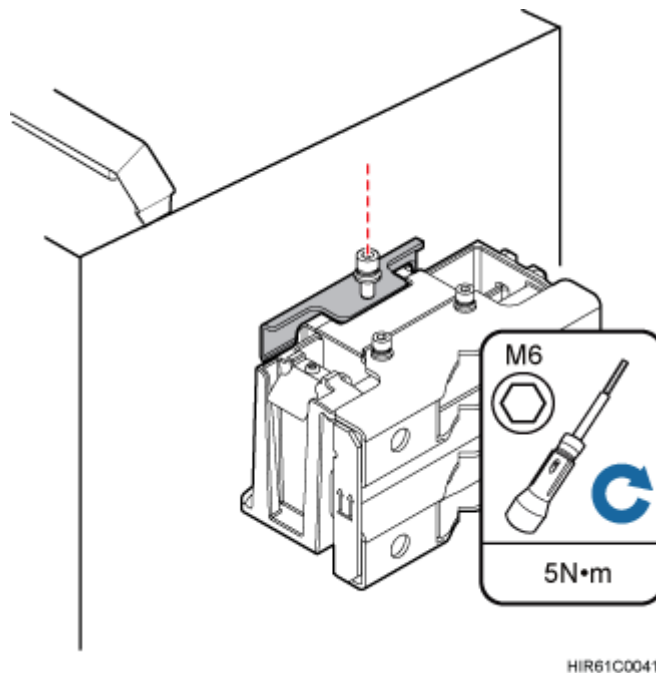
Figure 8-35 Securing the captive screw into the connection hole
