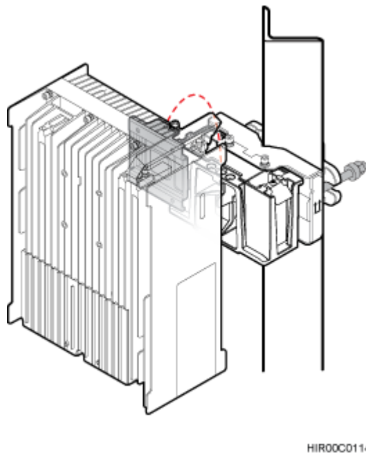
Figure 8-34 Installing the RRU onto the main bracket
