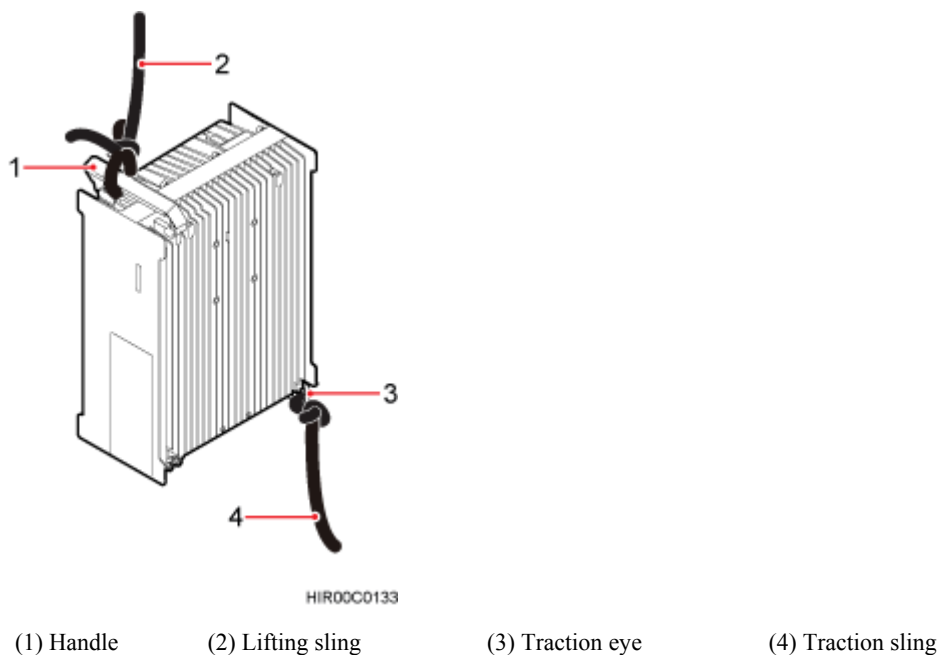
Figure 7-2 Binding the RRU
