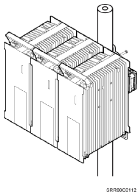
Figure 3-10 Three RRUs installed on a pole
