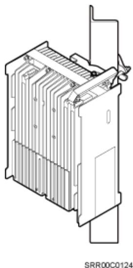
Figure 3-16 RRU installed on angle steel
