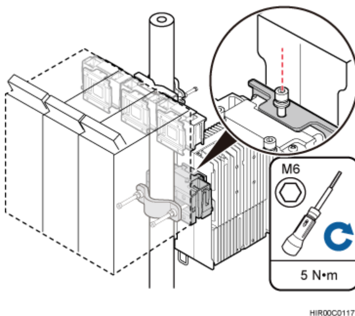
Figure 8-21 Installing the fourth RRU on the fourth main bracket
