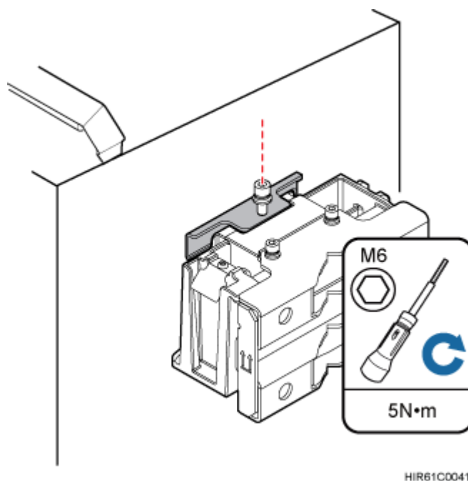
Figure 8-43 Securing the captive screw into the connection hole
