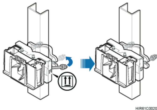
Figure 8-24 Installing the RRU mounting brackets
