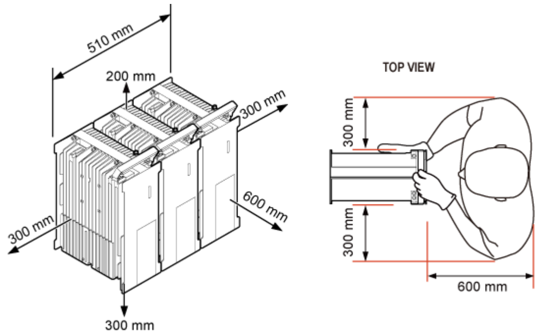
Figure 3-27 Minimum clearances for three or more RRUs installed in centralized mode
