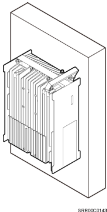
Figure 3-18 RRU installed on a wall
