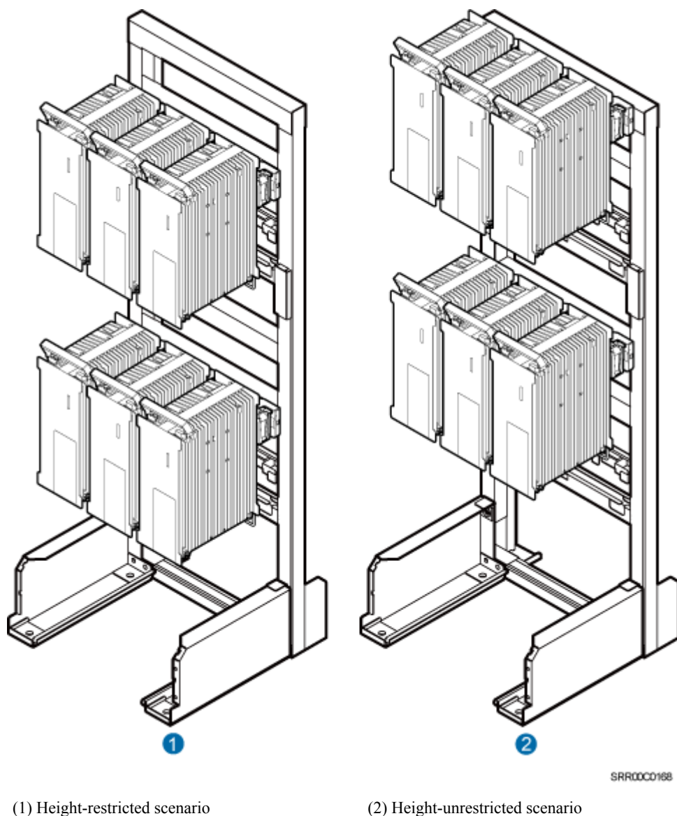
Figure 3-21 Six RRUs installed on an IFS06
