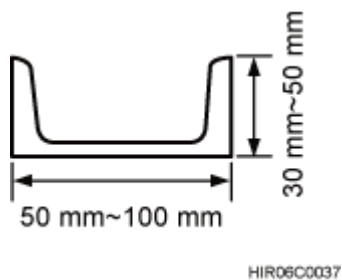
Figure 3-13 U-steel specifications
