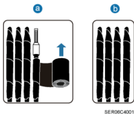
Figure 9-24 Method for handling cord end terminals that are not in use
