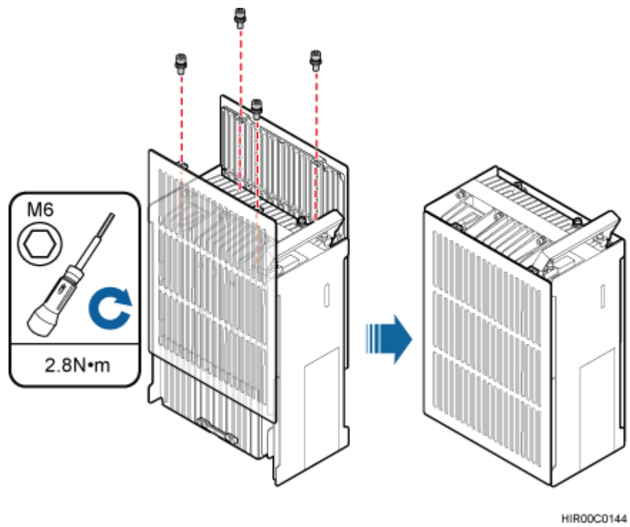
Figure 6-3 Installing the plastic shells of the RRU
