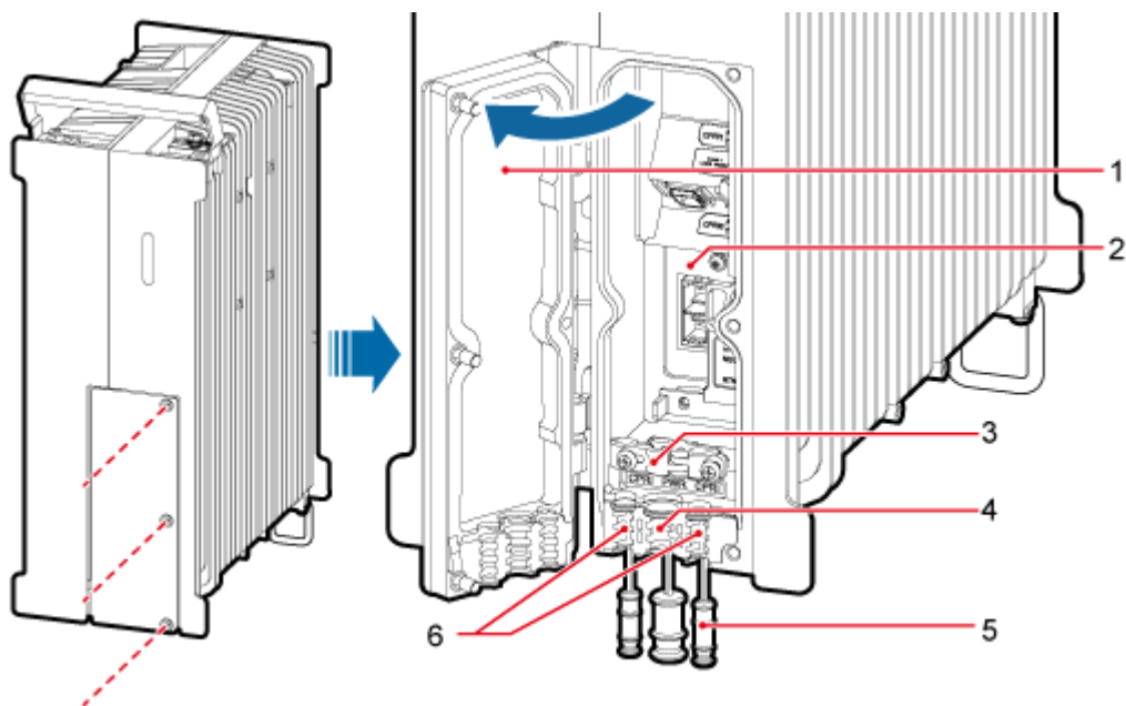
Figure 9-25 Opening the cover plate of the RRU cabling cavity
