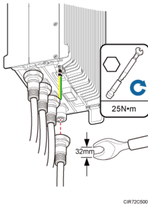
Figure 9-16 Installing an RRU RF jumper
