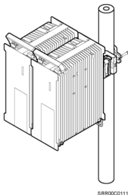
Figure 3-9 Two RRUs installed on a pole
