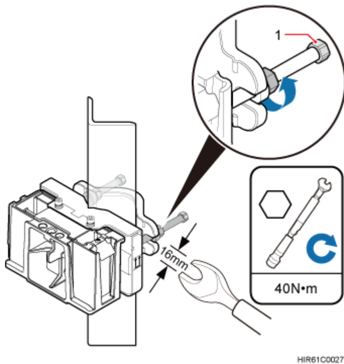
Figure 8-32 Securing the RRU mounting brackets
