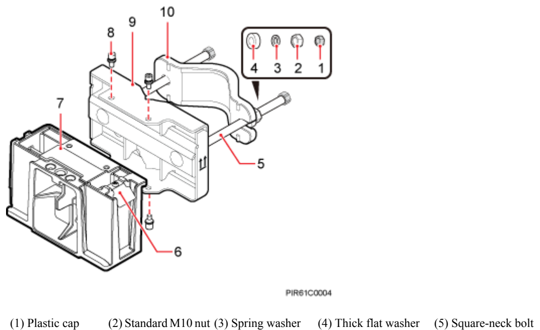
Figure 8-2 18 L blade RRU mounting kit
