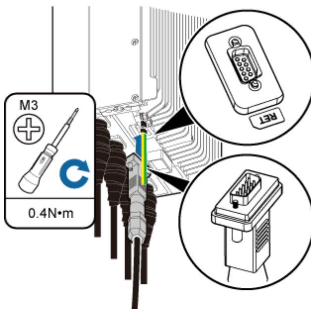
Figure 9-20 Installing an RRU AISG multi-wire cable
