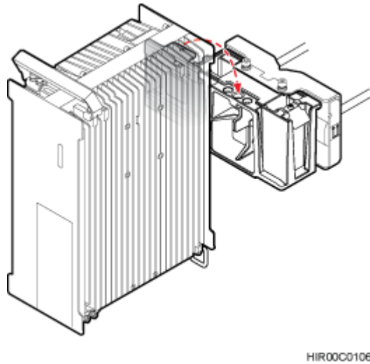
Figure 8-6 Installing the RRU onto the main bracket
