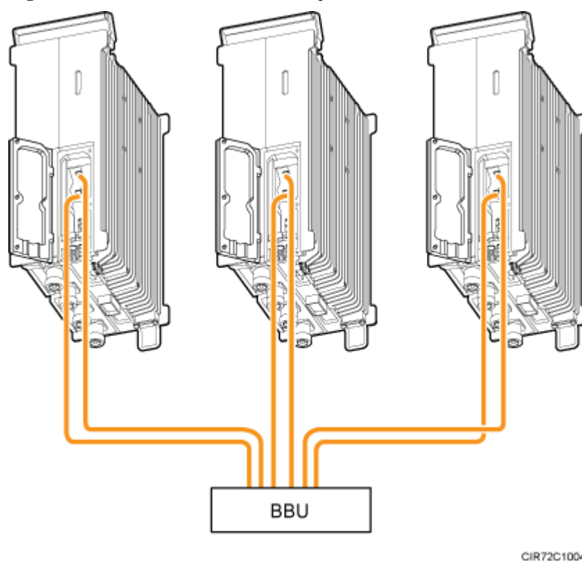
Figure 9-11 Cable connections of multiple multimode RRUs
