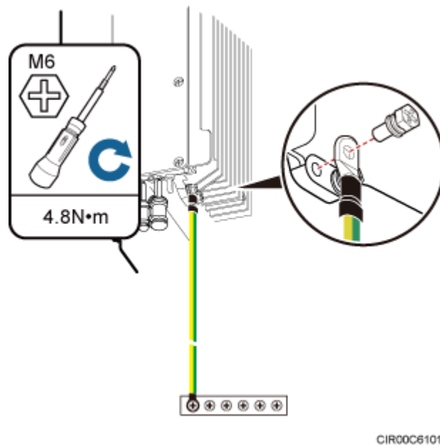
Figure 9-14 Installing an RRU PGND cable
