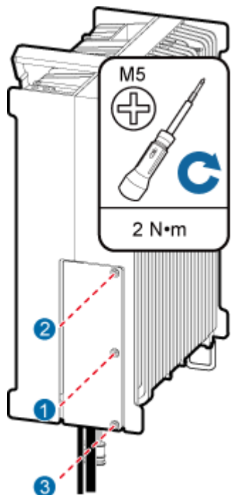
Figure 9-32 Closing the cover plate of an RRU cabling cavity
