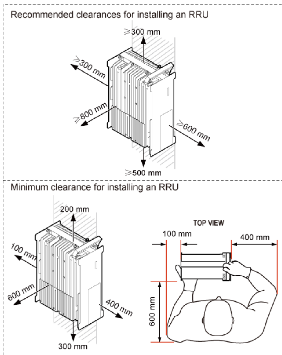
Figure 3-23 Clearance for a single RRU in standard or reverse mode
