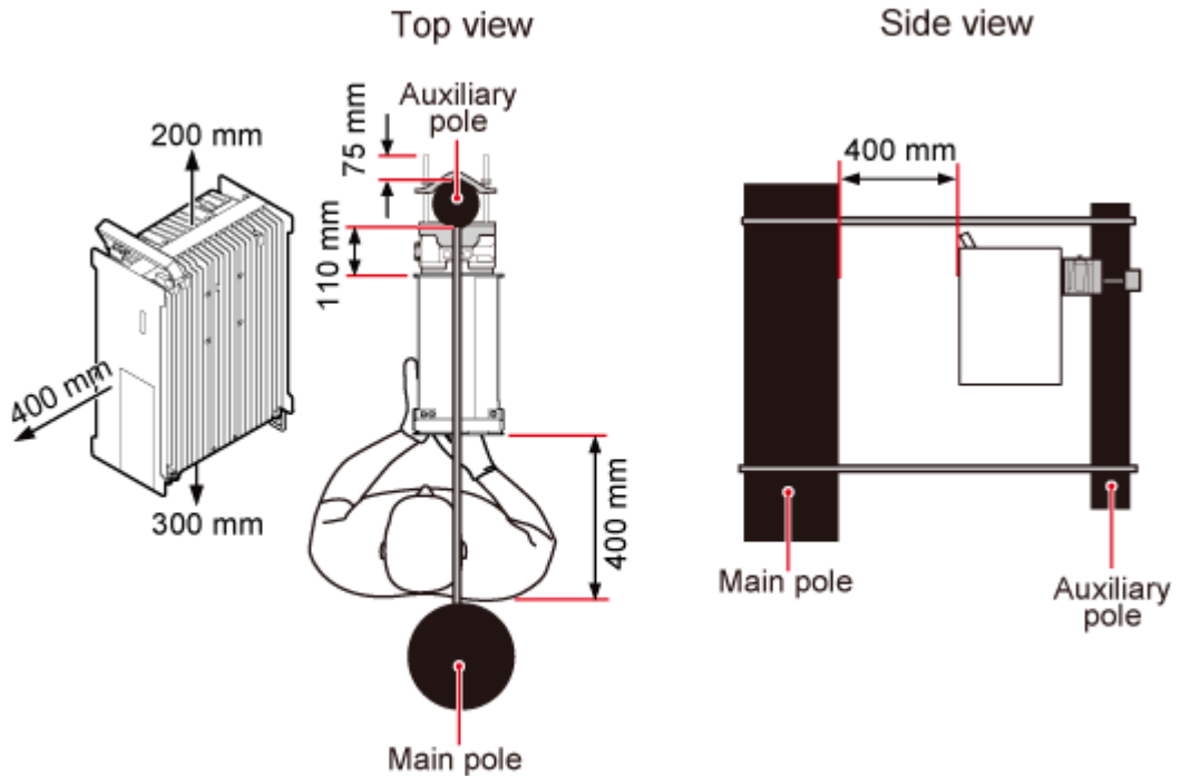
Figure 3-24 Minimum clearance for a single RRU in side-mounted mode on a tower
