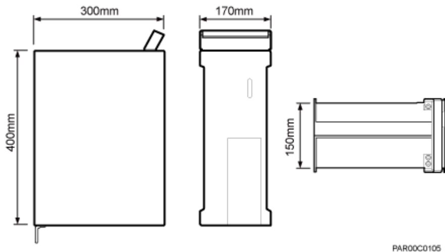
Figure 3-2 RRU dimensions
