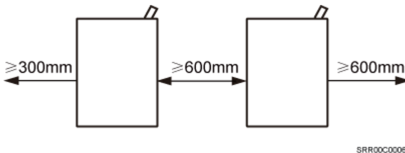
Figure 3-31 Recommended horizontal spacing between RRUs
