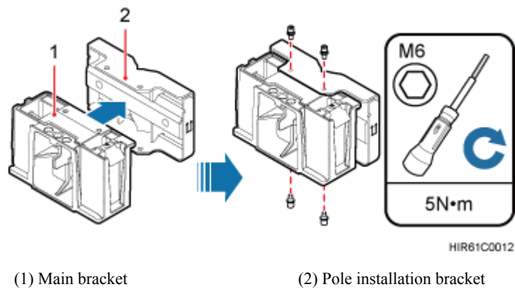
Figure 8-46 Installing the main bracket
