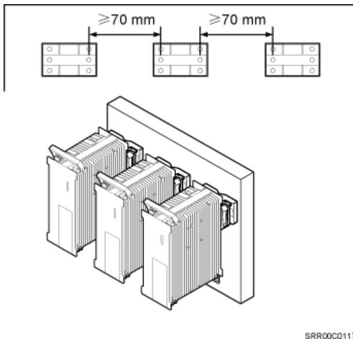
Figure 3-30 Recommended clearances for three or more RRUs installed in side-mounted mode on a wall
