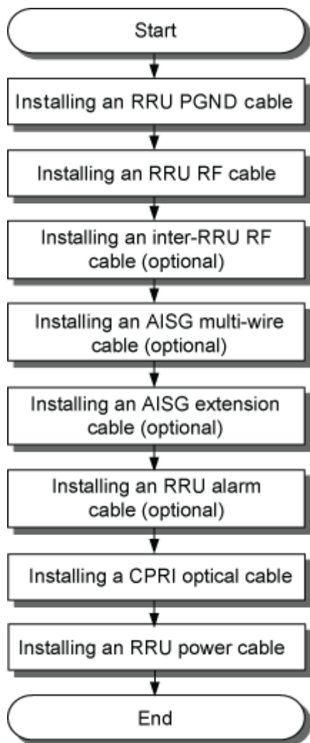
Figure 9-13 Procedure for installing RRU cables
