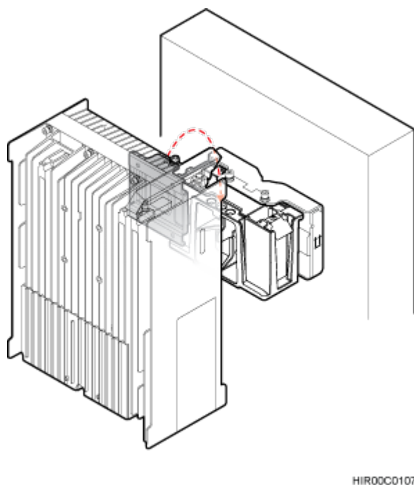
Figure 8-42 Installing the RRU onto the main bracket
