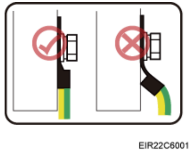
Figure 9-15 Correct position of an OT terminal
