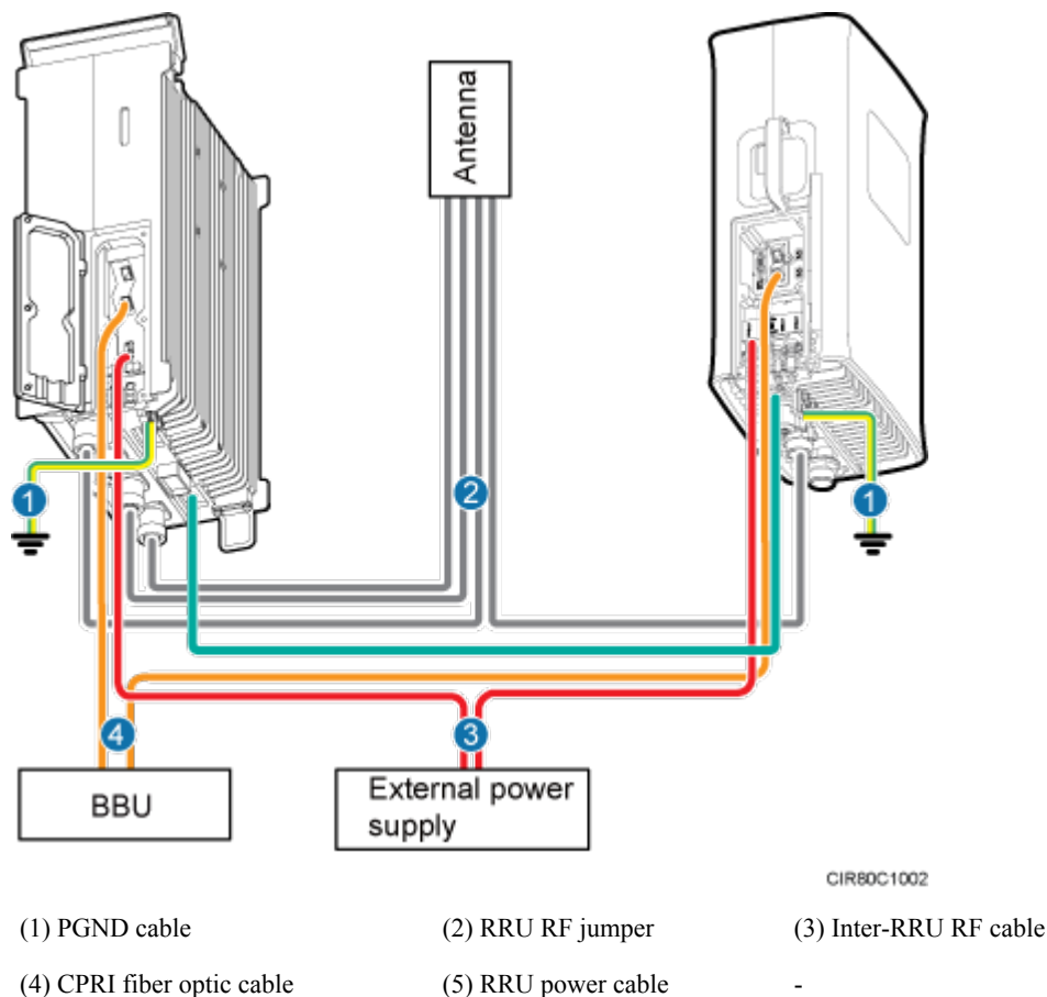
Figure 9-12 Inter-RRU cable connections
