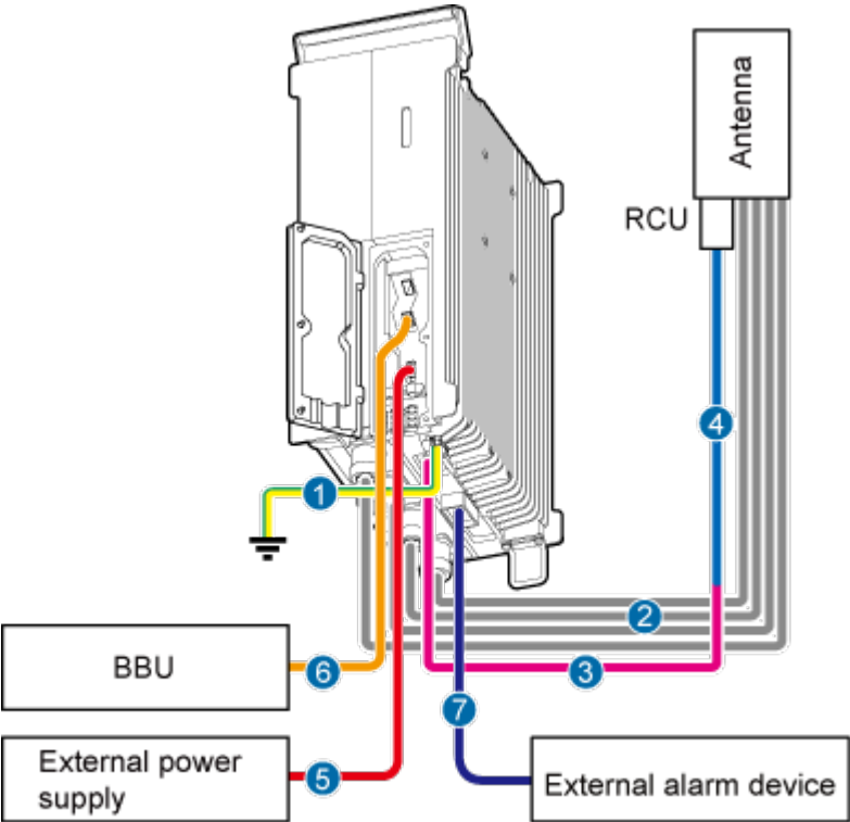
Figure 9-8 Cable connections of a single-mode RRU
