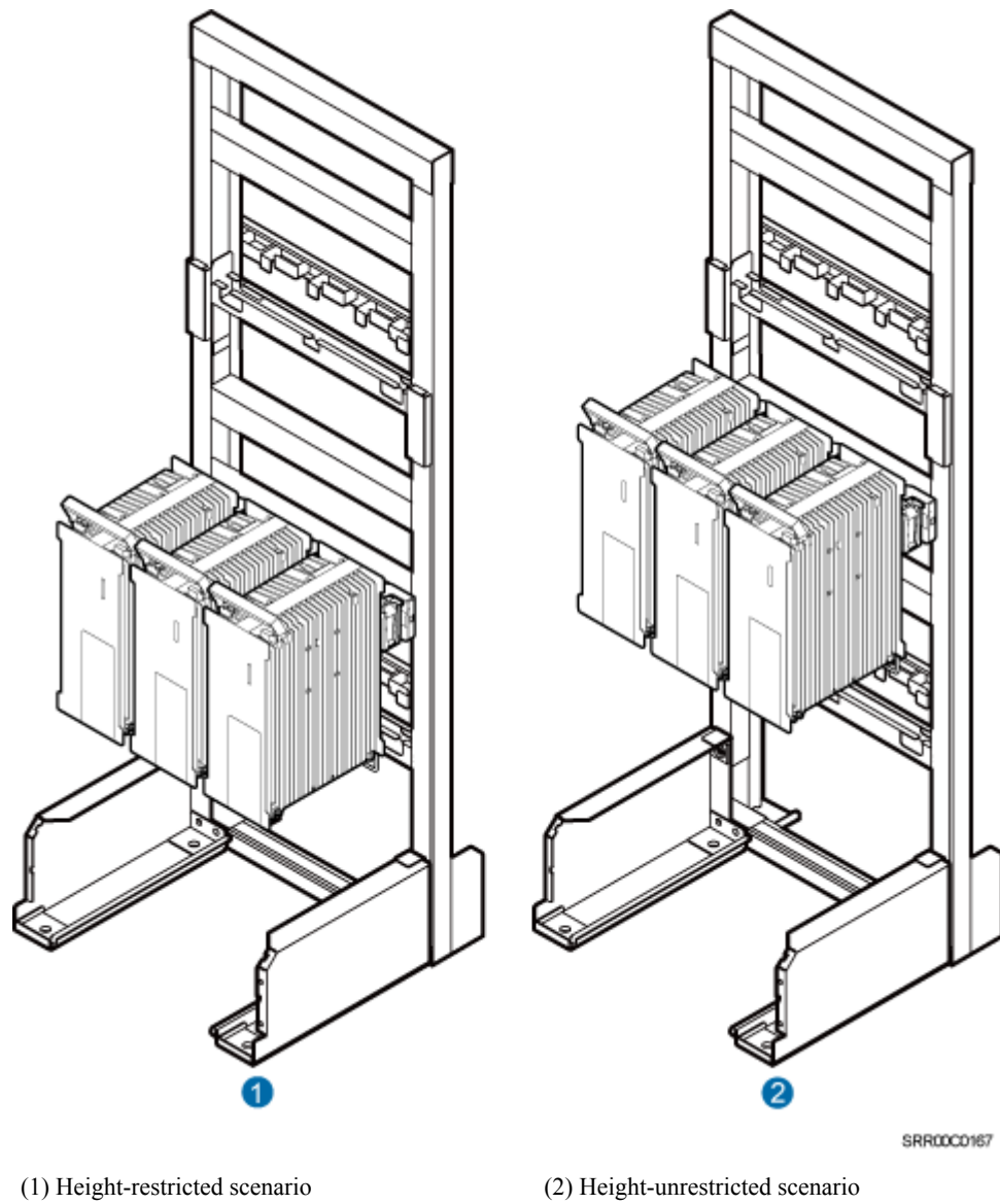
Figure 3-20 Three RRUs installed on an IFS06
