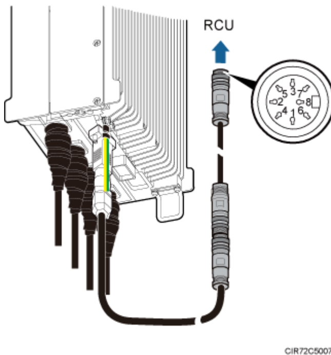
Figure 9-22 Installing an RRU AISG extension cable
