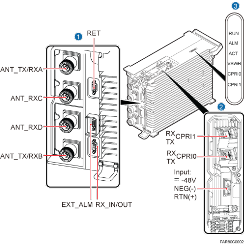
Figure 3-4 Ports on the RRU1 panels
