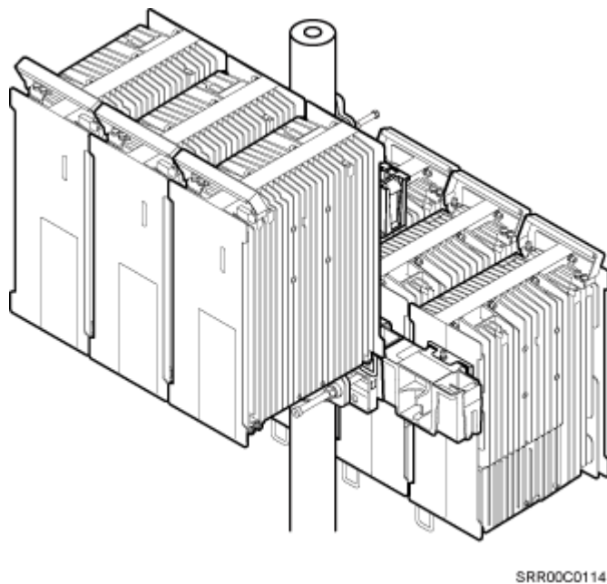
Figure 3-12 Six RRUs installed on a pole
