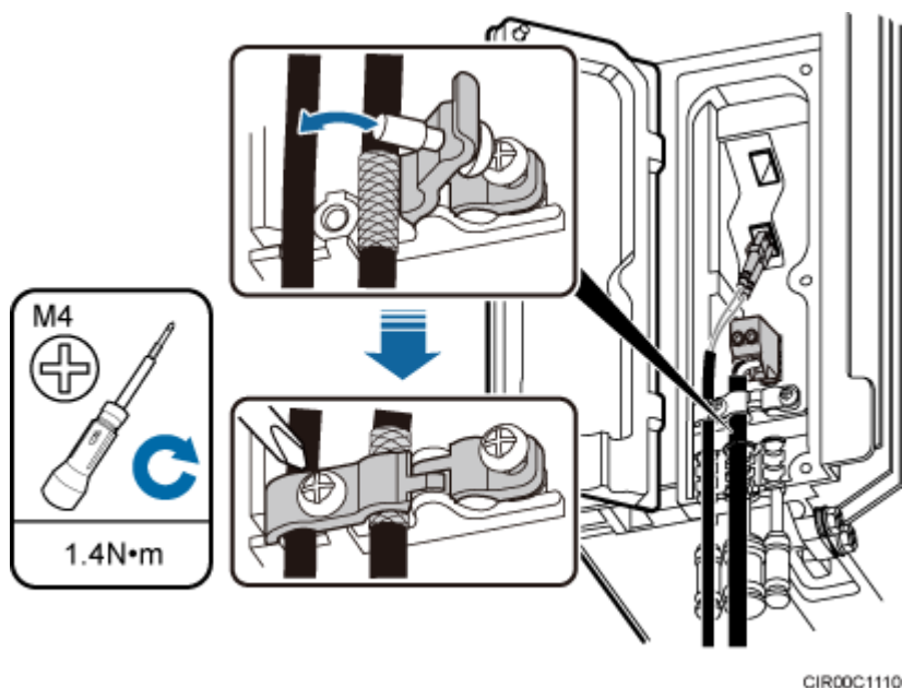
Figure 9-30 Closing clips
