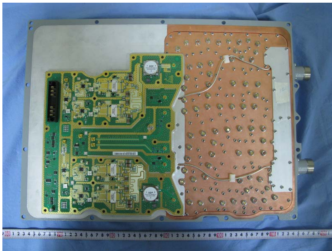
Photo-02 Internal Rear View –PA
