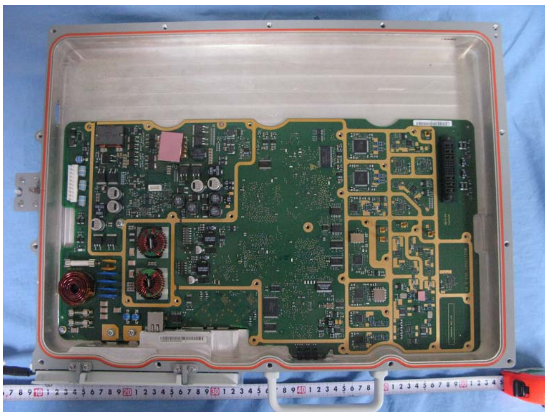
Photo-01 Internal Rear View –TRX
