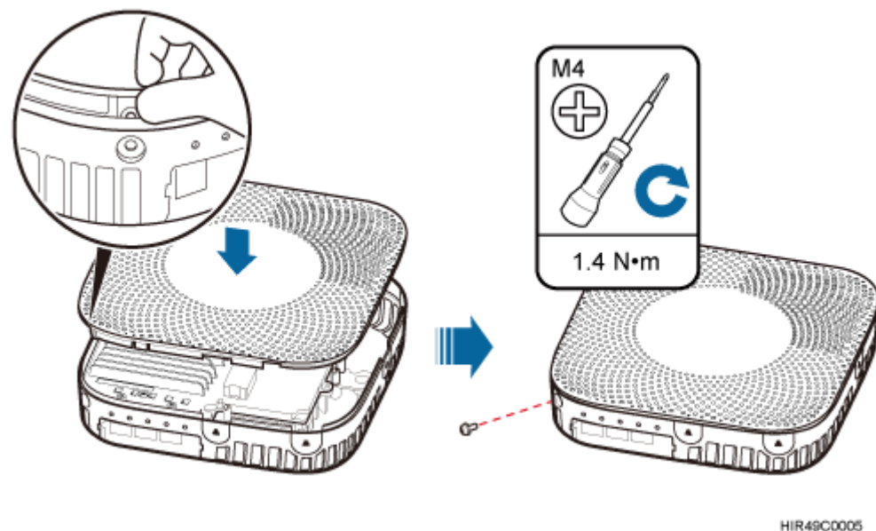
Figure 8-11 Installing the pRRU3901 housing
