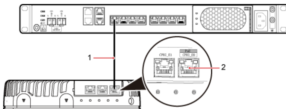
Figure 5-32 Install an Ethernet cable between an RHUB3908 and a pRRU3901
