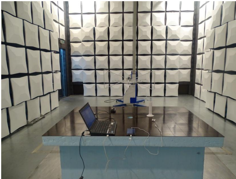
Radiated Spurious Emission (30MHz to 1GHz)
