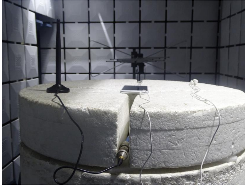
Radiated Spurious Emission (30M-3GHz)
