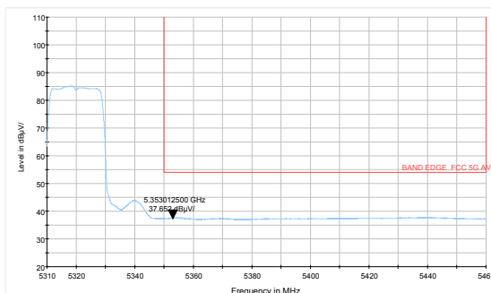
802.11ac VHT20 -Channel 64: Average
