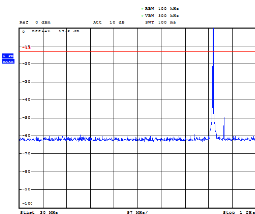
LTE Band 26 1.4MHz CH-High 30MHz~1GHz
