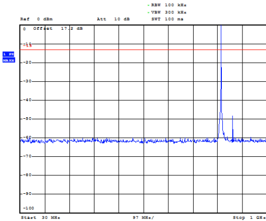
LTE Band 26 1.4MHz CH-High 30MHz~1GHz
