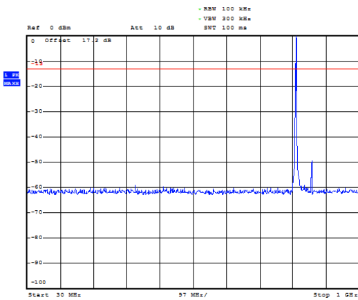
LTE Band 26 1.4MHz CH-Middle 30MHz~1GHz
