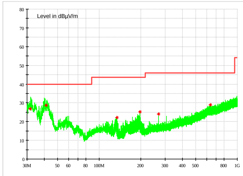
MEASUREMENT RESULT: QP Detector
