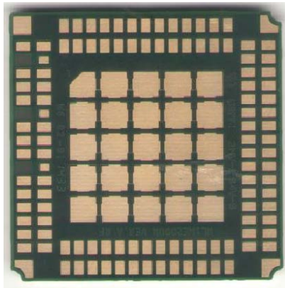
Figure1 EUT Appearance
