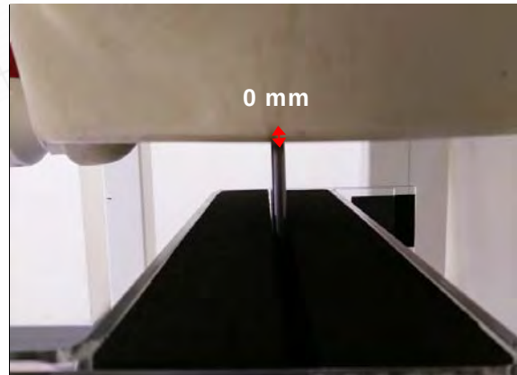
Fig.16 EUT Bottom side to flat phantom
