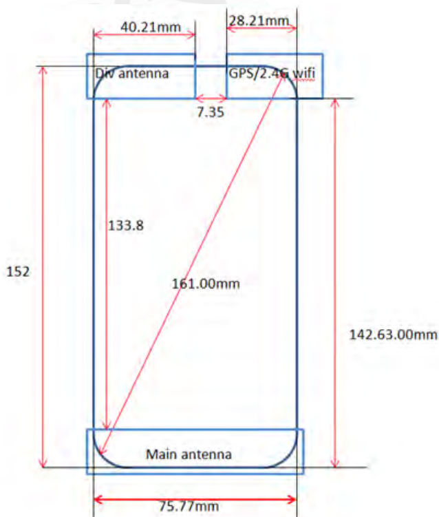
Fig.20 Antenna position of EUT
