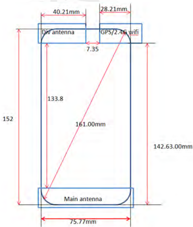
Fig.17 Antenna position of EUT
