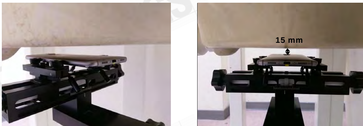
Fig.8 EUT Back side to flat phantom
