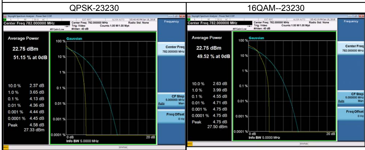
eMTC Band 13 Spectrum Plot_5M
