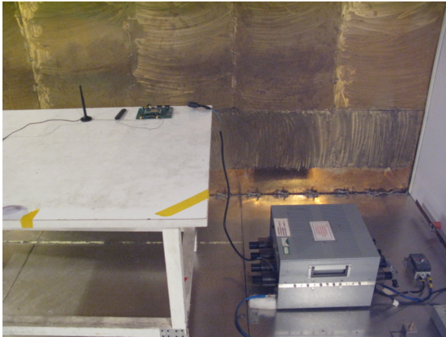
Conducted Emissions for AC
