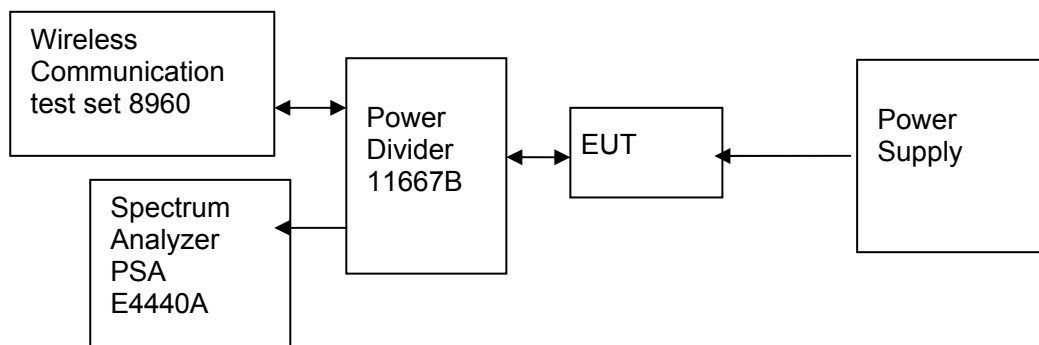
Figure 4. Test Set-up
