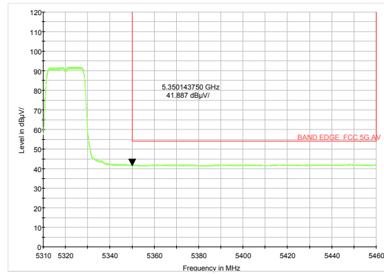
802.11a-Channel 64: Average
