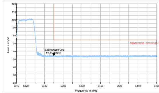
802.11a-Channel 64: Peak
