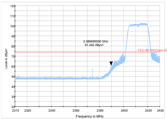
802.11g-Channel 1 Peak
