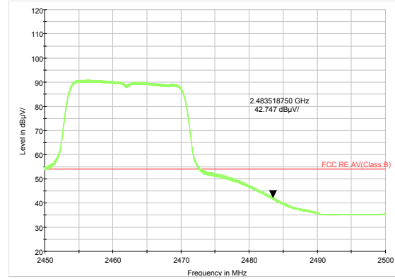
802.11g-Channel 11 Average
