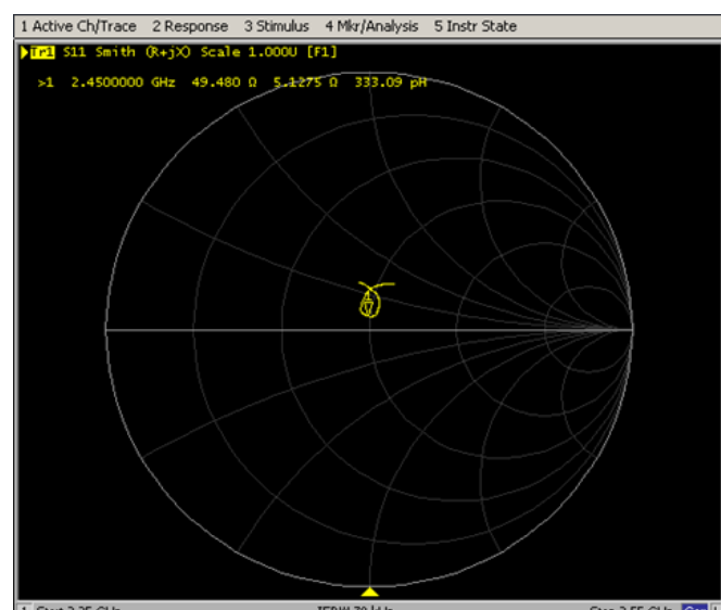
Impedance Test-Body
