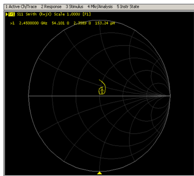
Impedance Test-Body
