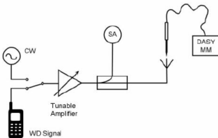
Fig. 6 Probe Modulation Factor Test Setup
