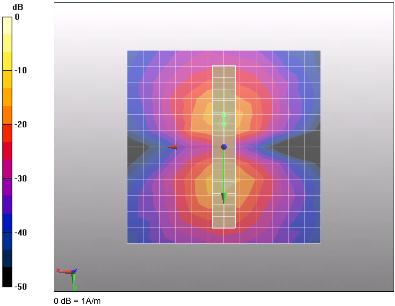
Figure 12 T-Coil CDMA Cellular Y transversal
