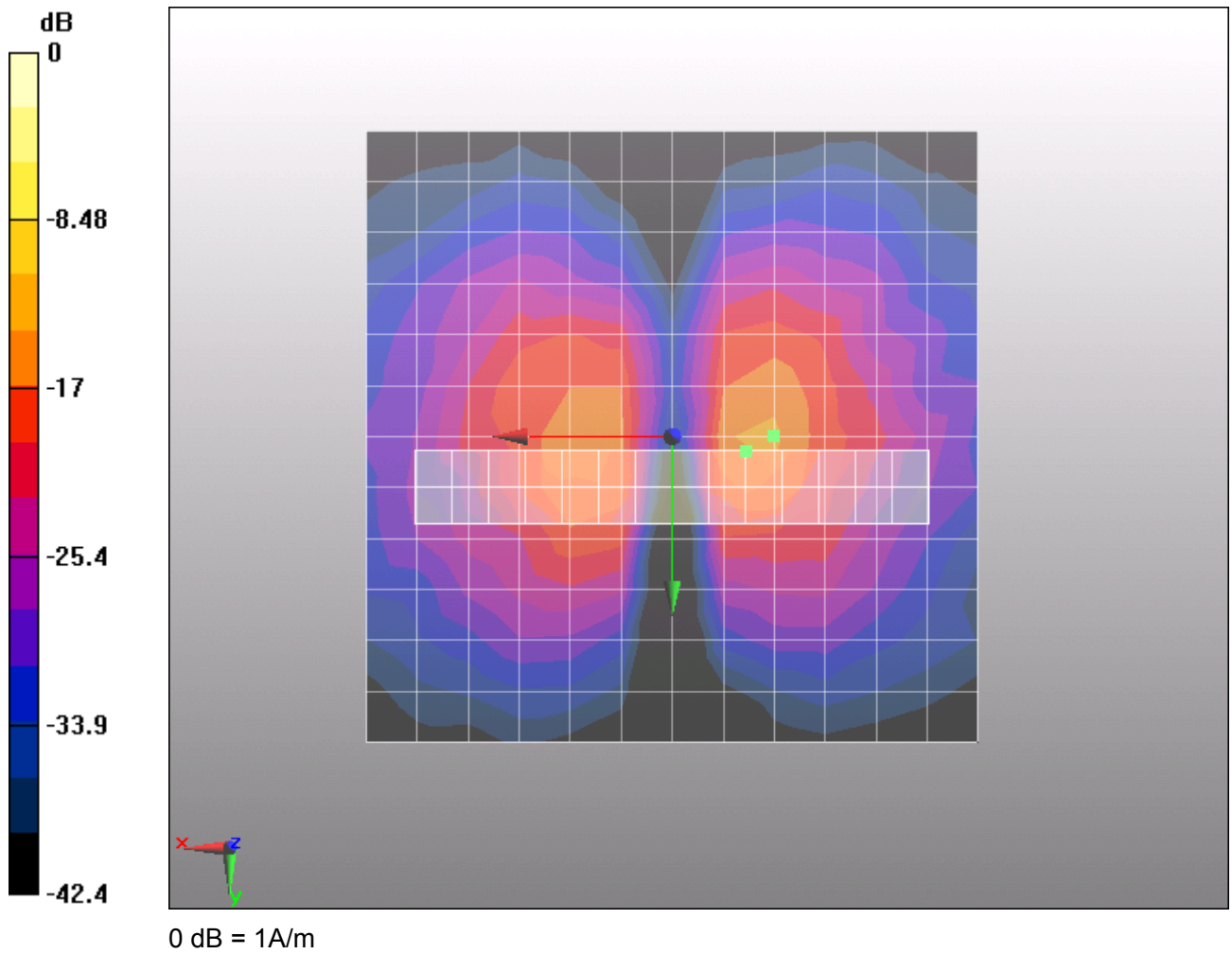
Figure 17 T-Coil CDMA PCS X longitudinal
