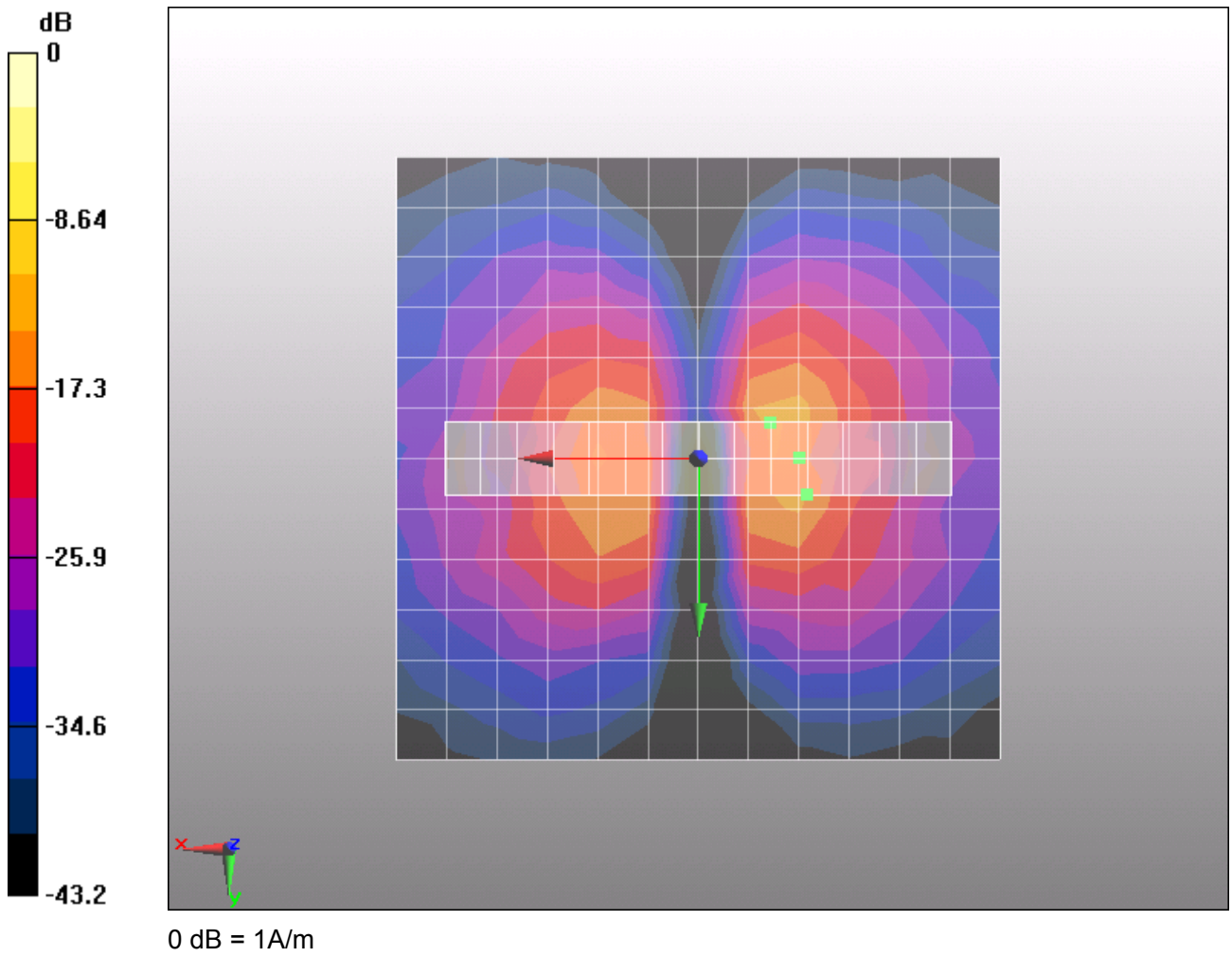
Figure 23 T-Coil CDMA AWS X longitudinal
