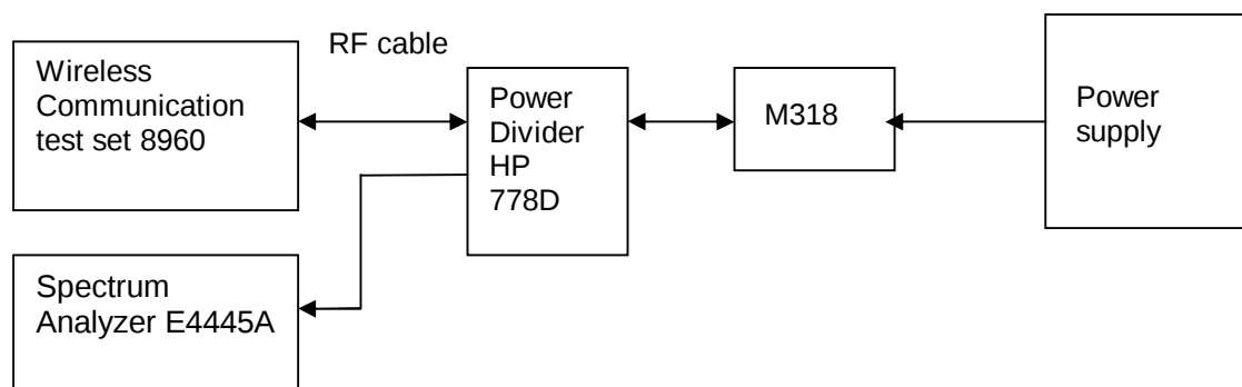
Figure 5. Test Set-up
