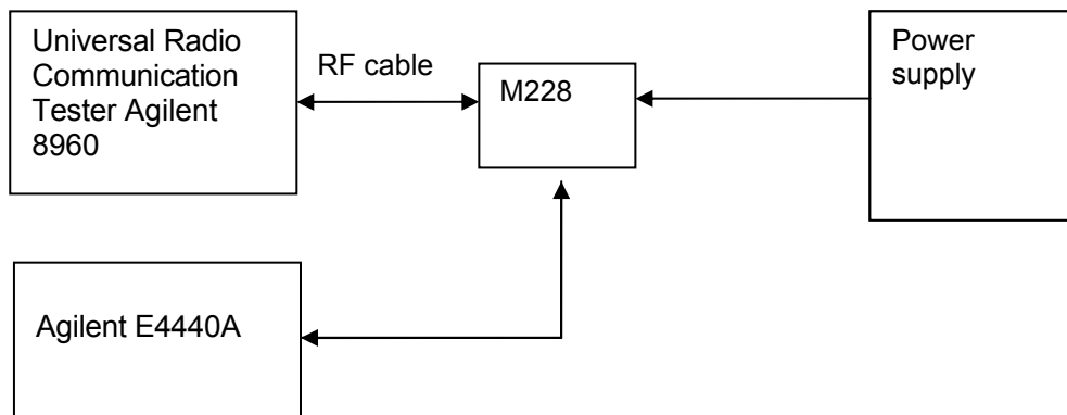
Figure 2. Test Set-up
