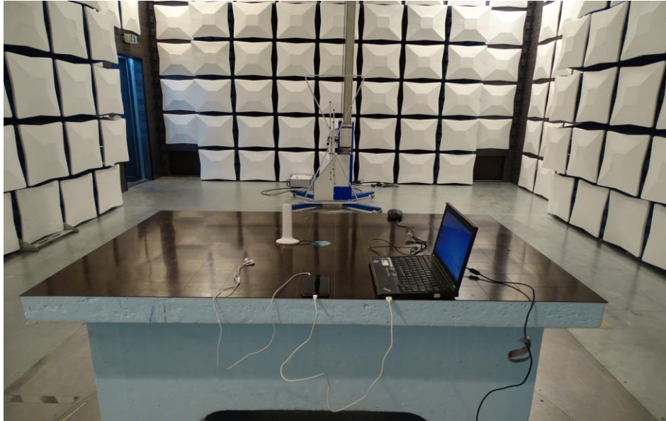
Radiated Spurious Emission (below 1GHz)
