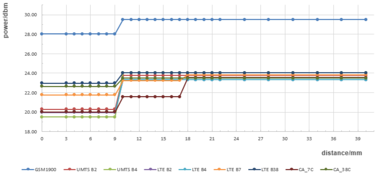
Distance VS Output Power Plot(Bottom)
