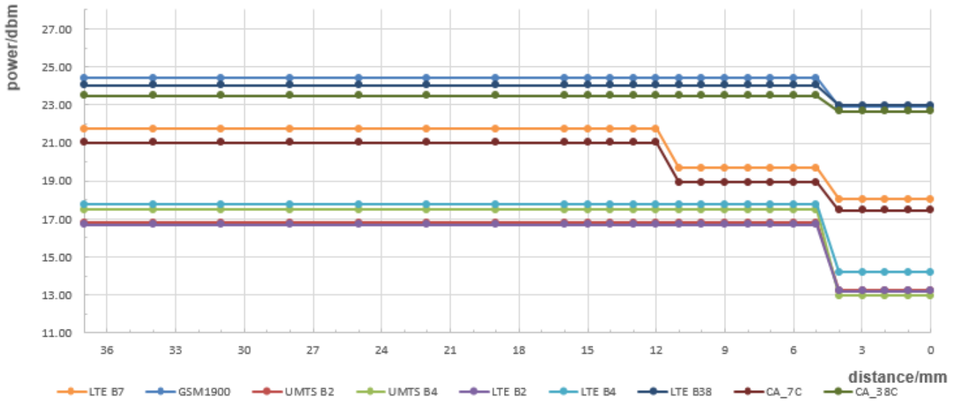
Distance VS Output Power Plot(Front)
