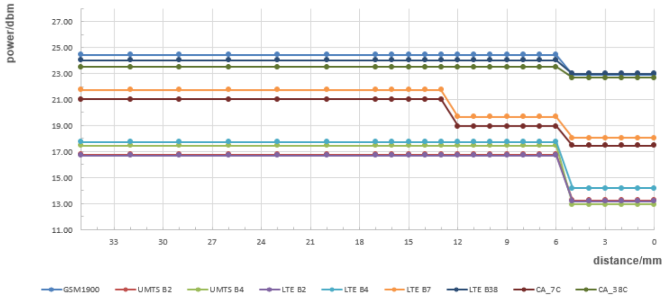
Distance VS Output Power Plot(Back)
