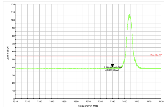
BT UHD 2M 8DPSK_2404MHz: Average
