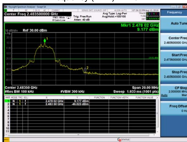
BT UHD 2M 8DPSK CH37, Carrier frequency (MHz): 2478
