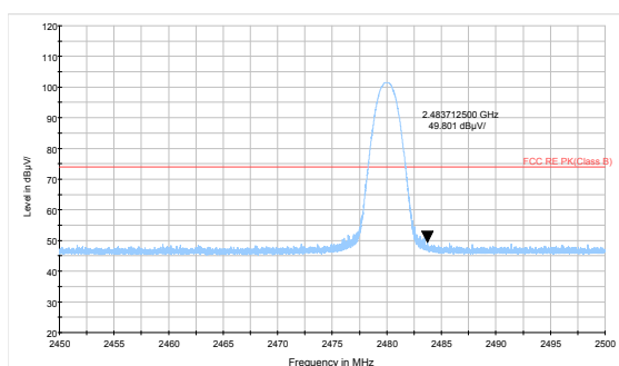
DH5-Channel 78: Peak
