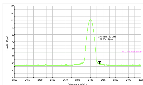
DH5-Channel 78: Average
