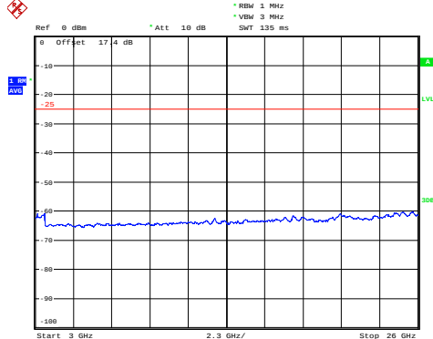
LTE Band 7 5MHz CH-Low 3GHz~26GHz
