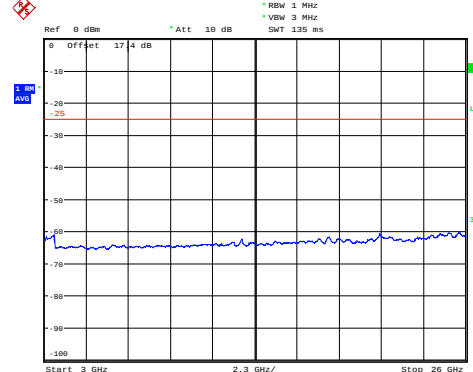
LTE Band 7 5MHz CH-Middle 3GHz~26GHz
