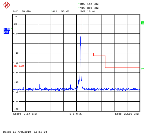
LTE Band 7 QPSK 10MHz CH-High, 1 RB
