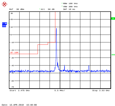
LTE Band 7 QPSK 10MHz CH-Low, 1 RB
