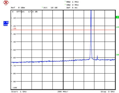
LTE Band 7 5MHz CH-Middle 1GHz~3GHz
