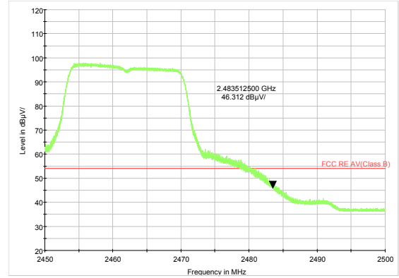
802.11g-Channel 11 Average
