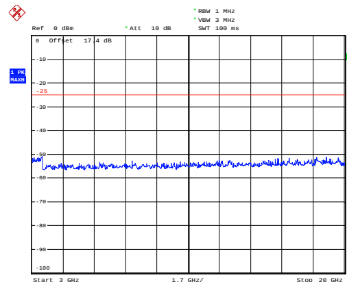
LTE Band 7 5MHz CH-Middle 3GHz~20GHz
