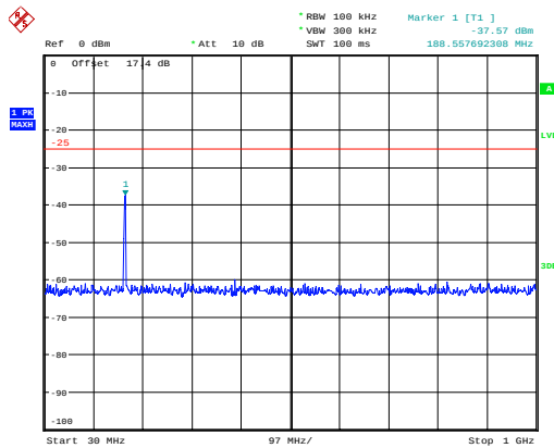
LTE Band 7 5MHz CH-Low 30MHz~1GHz
