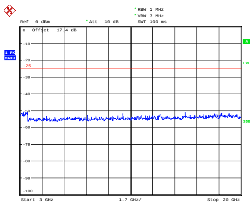
LTE Band 7 5MHz CH-Low 3GHz~20GHz
