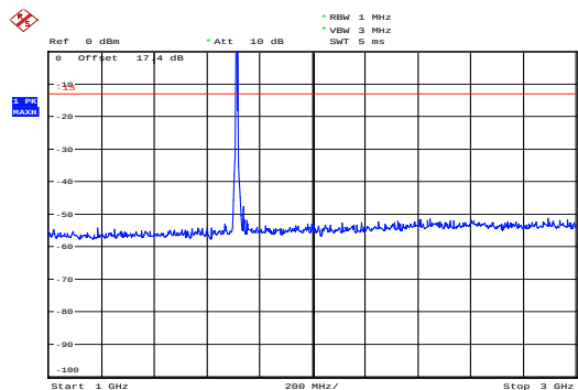
WCDMA Band IV CH-Low 1GHz ~3GHz
