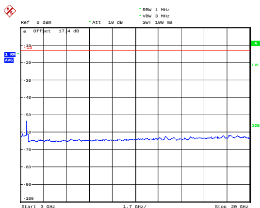
LTE Band 4 1.4MHz CH-Low 3GHz~20GHz
