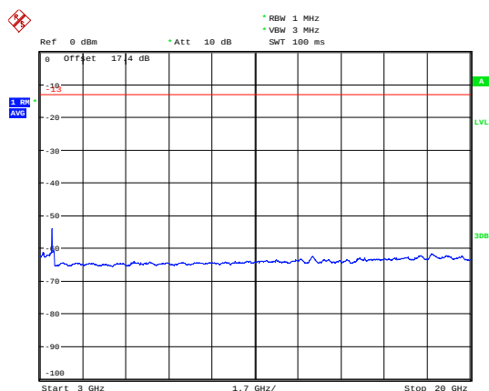
LTE Band 4 1.4MHz CH-Middle 3GHz~20GHz
