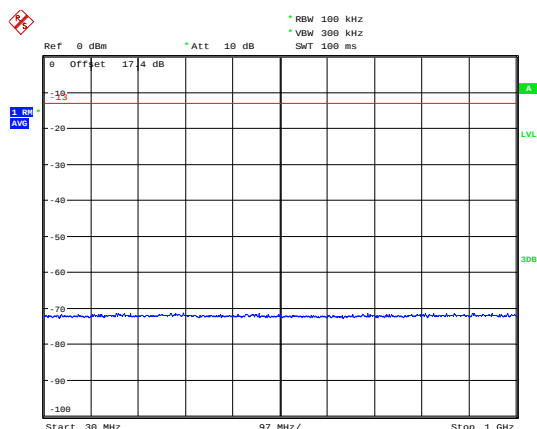
LTE Band 4 10MHz CH-Low 30MHz~1GHz
