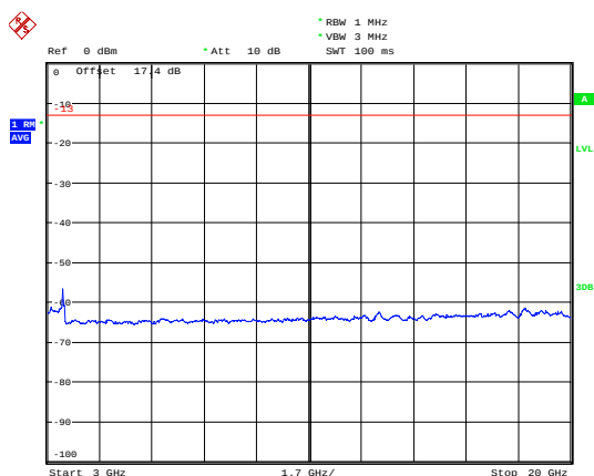
LTE Band 4 5MHz CH-High 3GHz~20GHz
