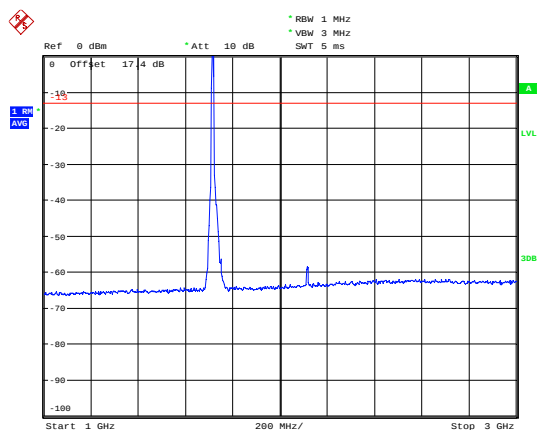
LTE Band 4 10MHz CH-Low 1GHz~3GHz
