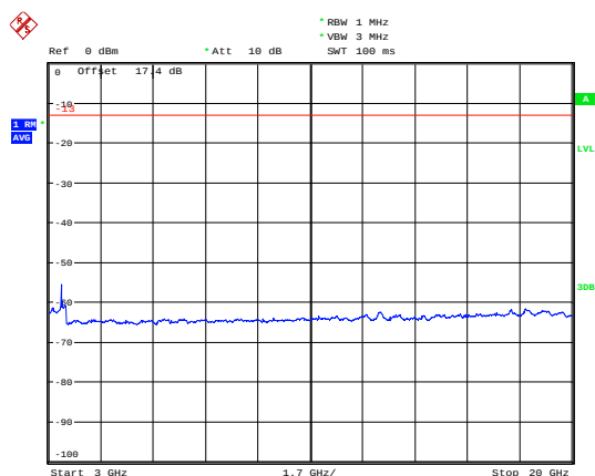
LTE Band 4 10MHz CH-Low 3GHz~20GHz
