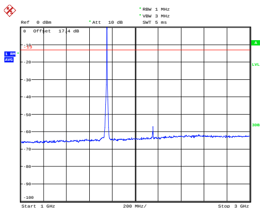
LTE Band 4 5MHz CH-High 1GHz~3GHz
