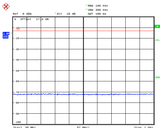
LTE Band 4 5MHz CH-High 30MHz~1GHz
