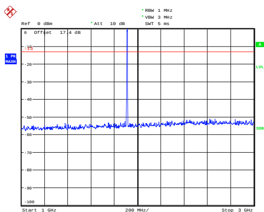
GSM 1900 CH-High 1GHz~3GHz
