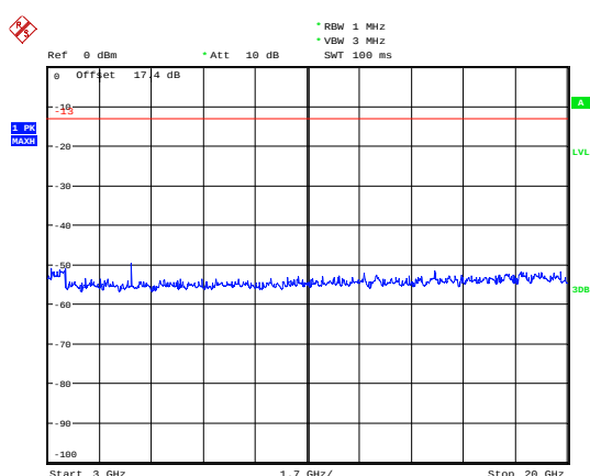
GSM 1900 CH-High 3GHz~20GHz
