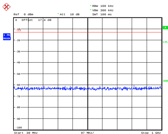
GSM 1900 CH-High 30MHz~1GHz
