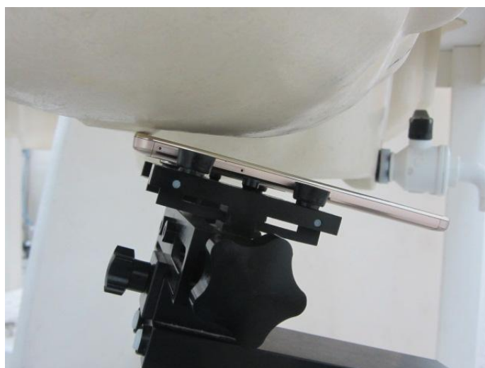
Photo 11: Back Side 15mm(KIW-L23)
