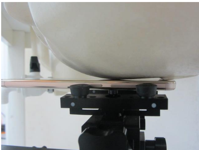
Photo 6: Left hand touch cheek(KIW-L23)
