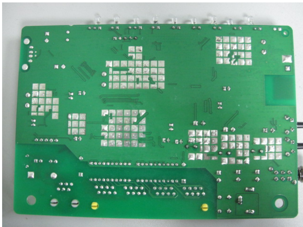
(5) EUT Photo(HG530)
