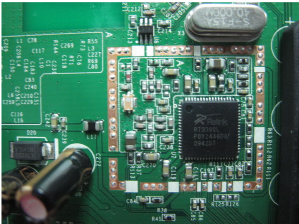
(3) EUT Photo(HG530)
