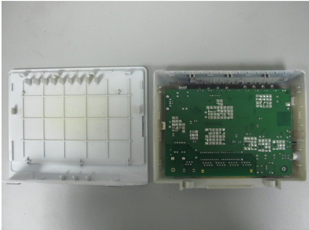
(2) EUT Photo(HG530)
