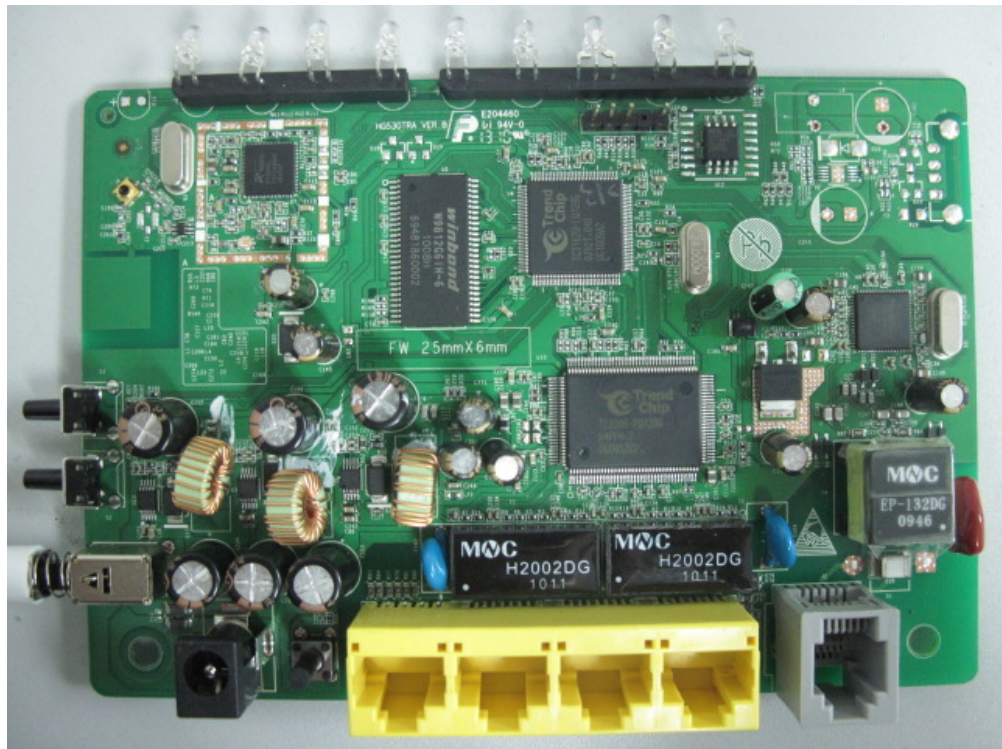
(4) EUT Photo (HG530)
