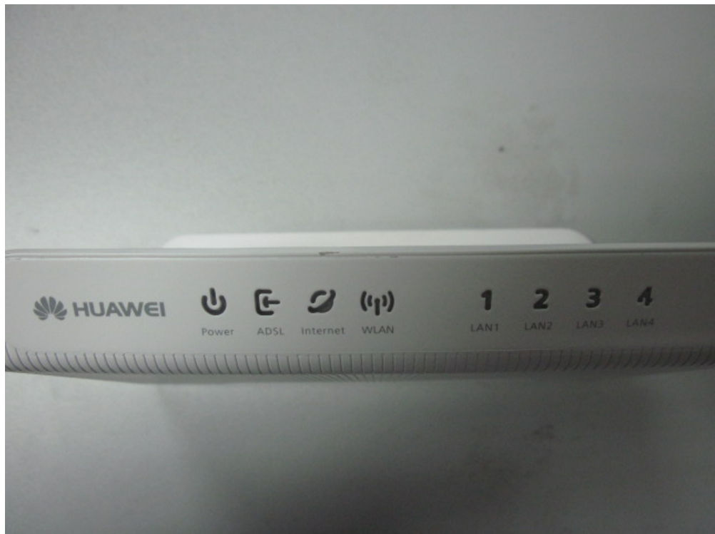
(4) EUT Photo(HG530)
