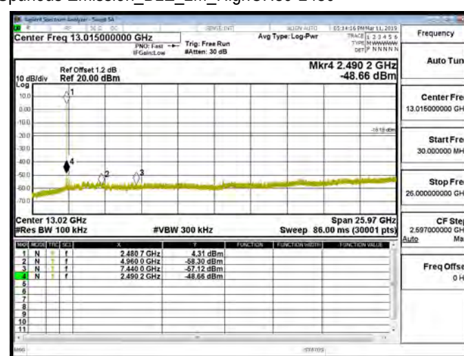
Spurious Emission_BLE_2M_HighCH39-2480
