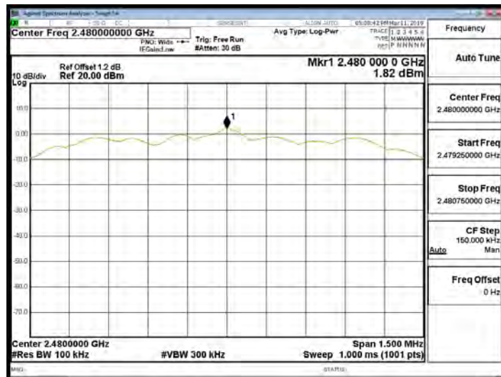
Reference Level_BLE_2M_HighCH39-2480
