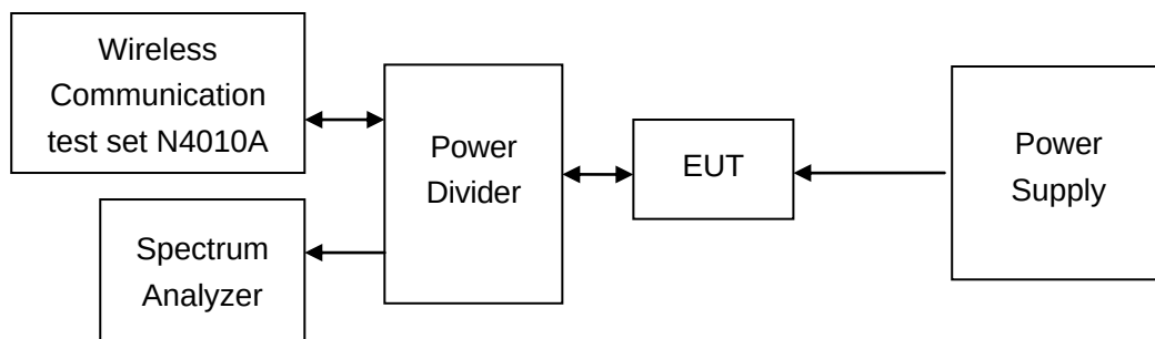
Figure 6. Test Set-up
