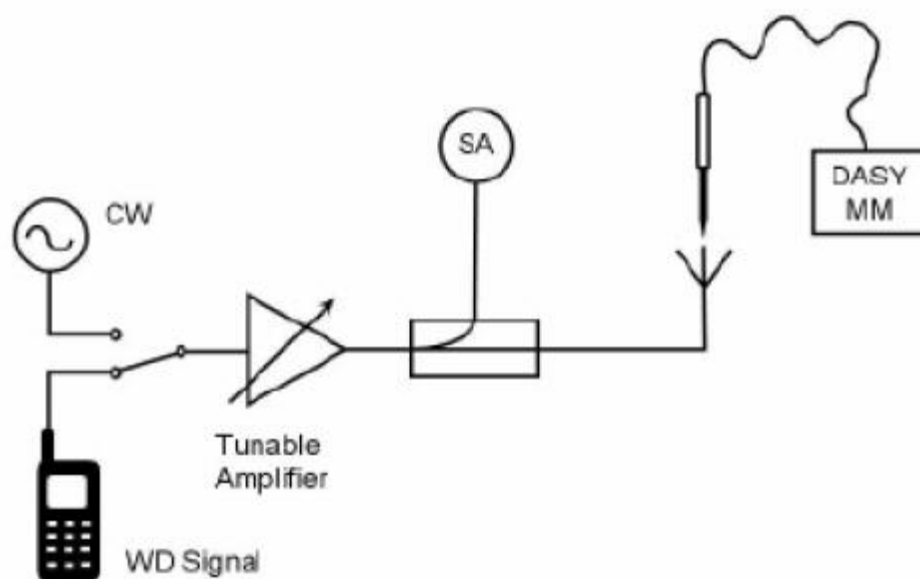
Fig. 6 Probe Modulation Factor Test Setup
