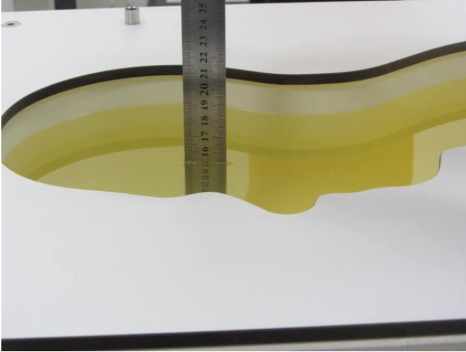
Photo 24: HSL835MHz Depth (15.1cm)
