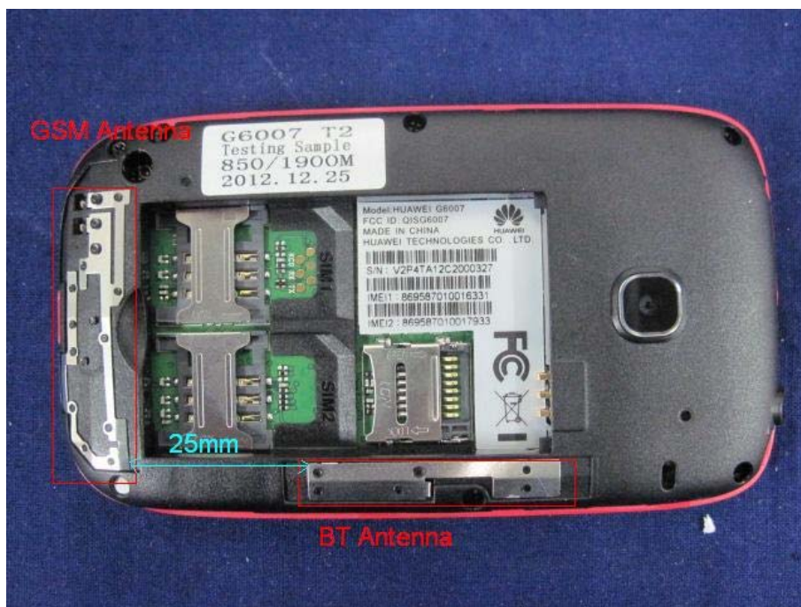
(14) EUT Photo for SAR
