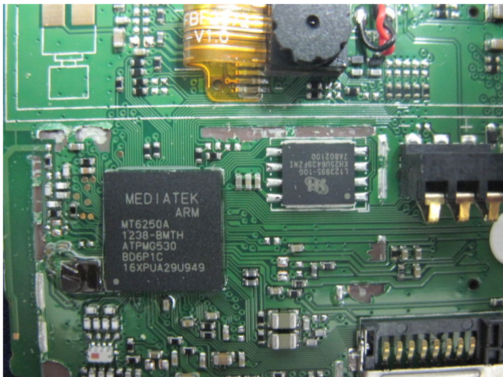
(12) EUT Photo (Single SIM Slot)
