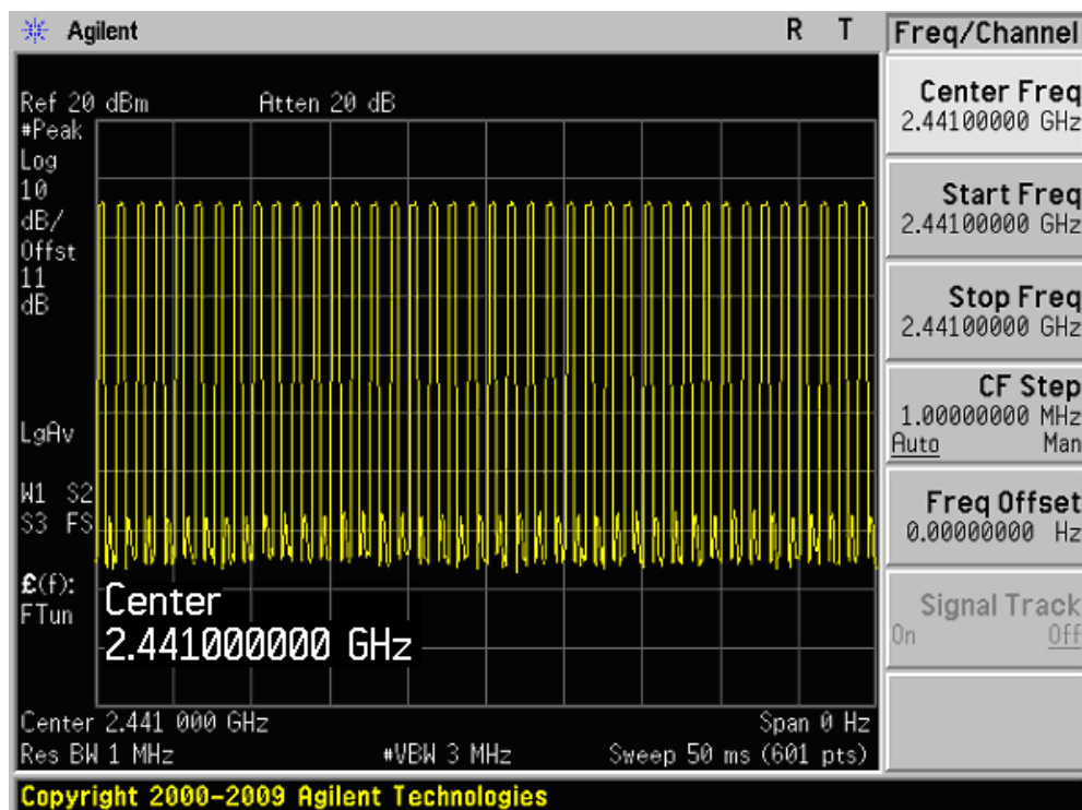
Channel 39 (2441MHz)-(3DH1)
