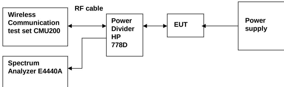
Figure 5. Test Set-up
