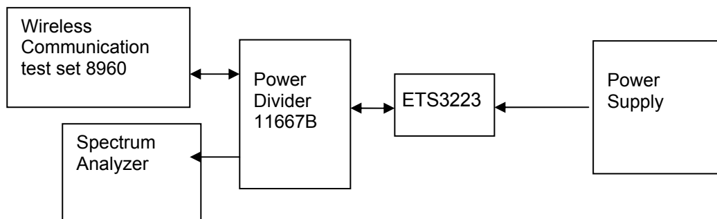
Figure 4. Test Set-up
