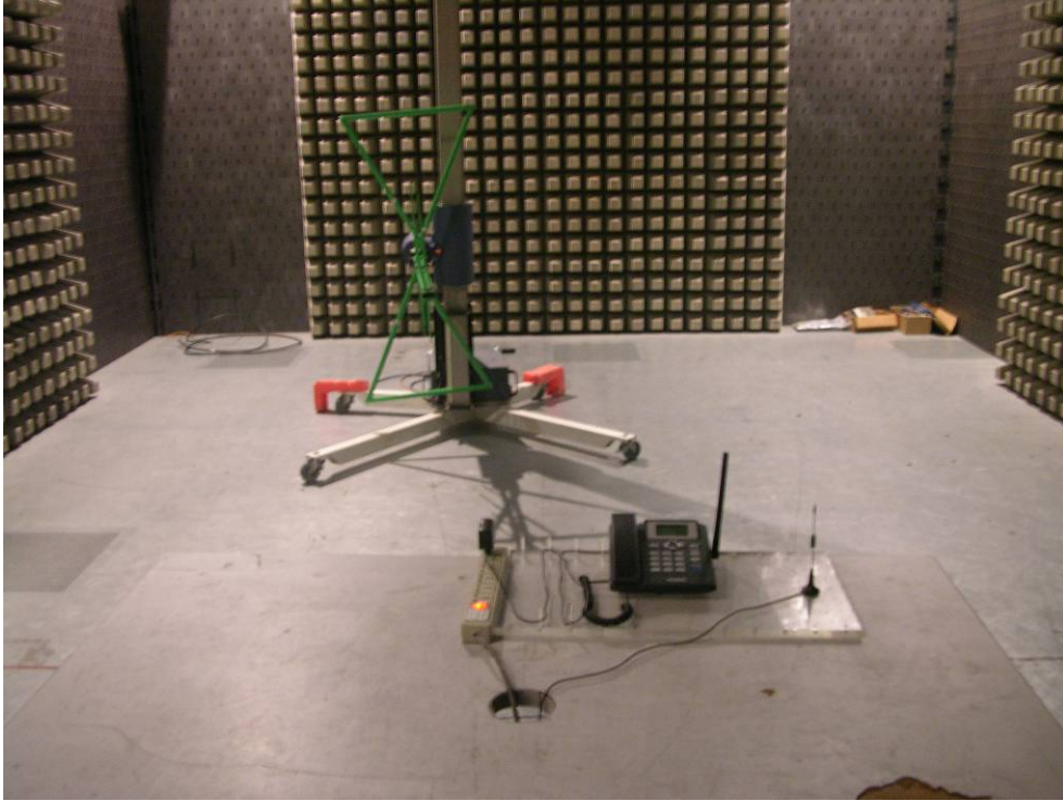
Radiated Disturbance
