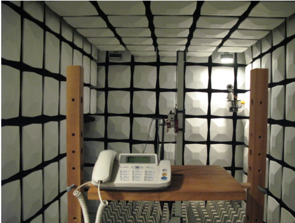
Radiated Spurious Emission (2GHz to26.5GHz)
