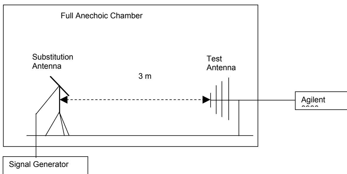
Figure 1. Test Set-up
