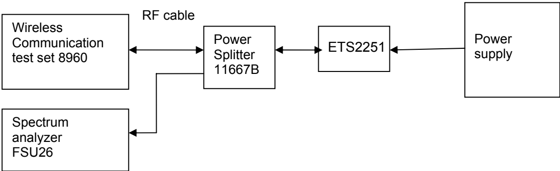
Figure 4. Test Set-up
