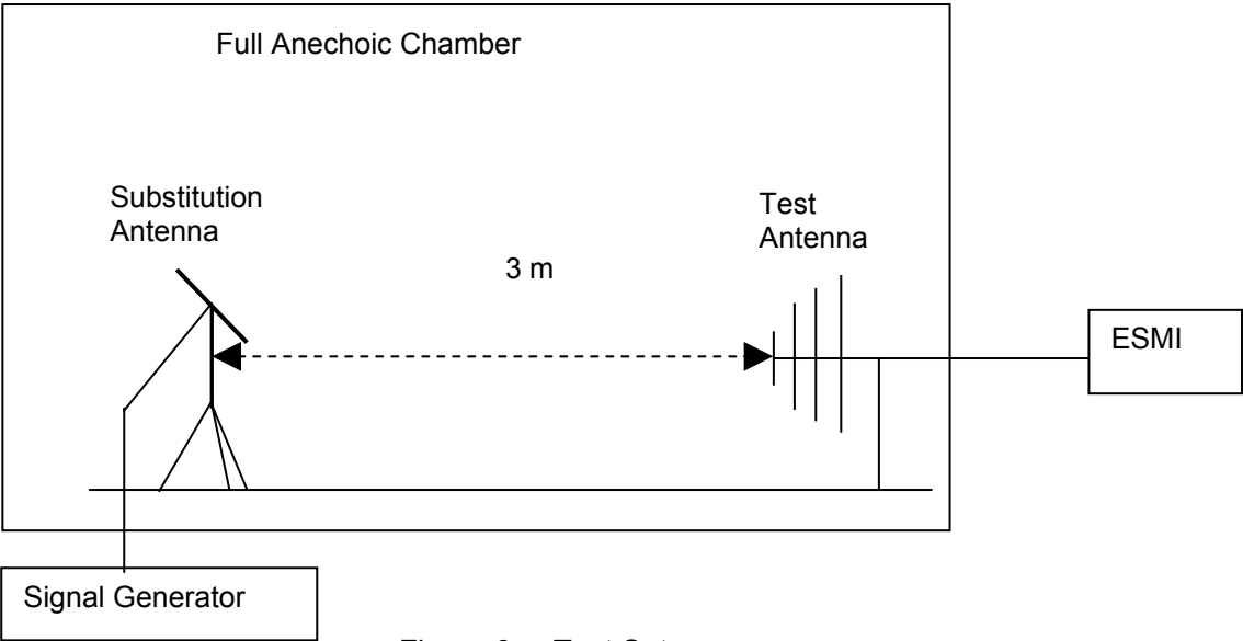
Figure 6. Test Set-up
