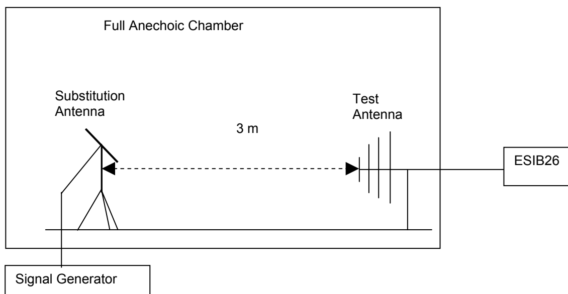
Figure 7. Test Set-up
